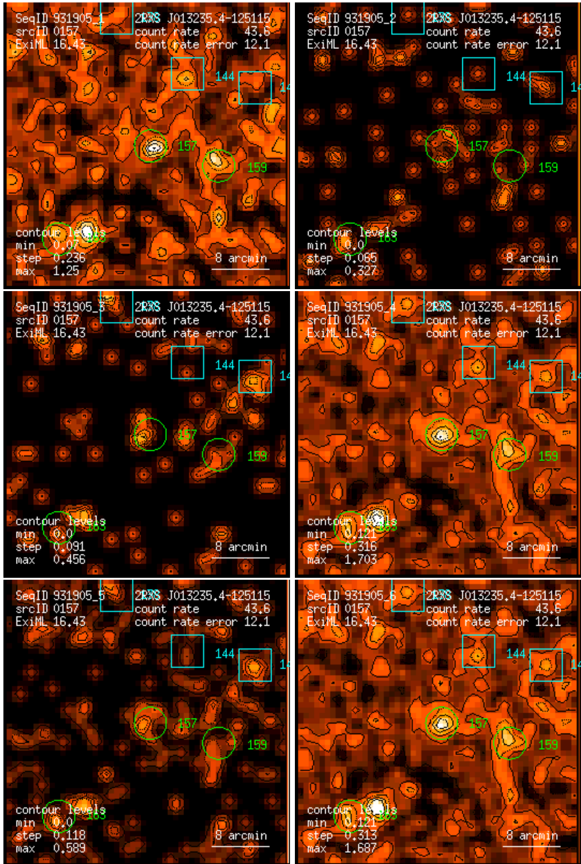
Figure 157: RASS 931905: detection 0157: band rate images, Gaussian filter: (1) PSPC channels 11 – 41, (2) 52 – 90, (3) 91 – 201, (4) 11 – 235, (5) 52 – 201, (6) 11 – 201. Broad band rates in counts/ks. Band rate contour levels in counts/ks/arcmin 2 .
