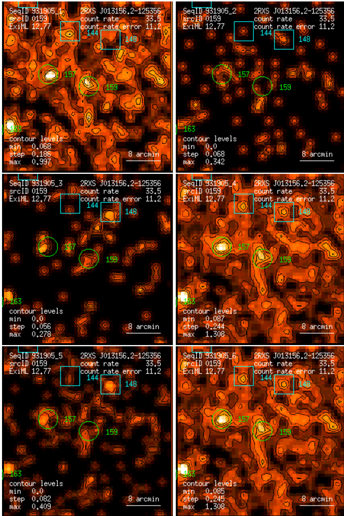
Figure 159: RASS 931905: detection 0159: band rate images, Gaussian filter: (1) PSPC channels 11 – 41, (2) 52 – 90, (3) 91 – 201, (4) 11 – 235, (5) 52 – 201, (6) 11 – 201. Broad band rates in counts/ks. Band rate contour levels in counts/ks/arcmin 2 .
