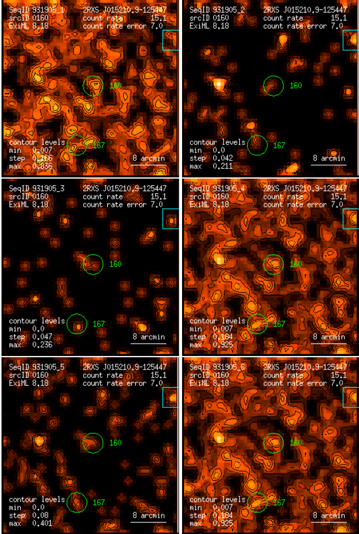
Figure 160: RASS 931905: detection 0160: band rate images, Gaussian filter: (1) PSPC channels 11 – 41, (2) 52 – 90, (3) 91 – 201, (4) 11 – 235, (5) 52 – 201, (6) 11 – 201. Broad band rates in counts/ks. Band rate contour levels in counts/ks/arcmin 2 .
