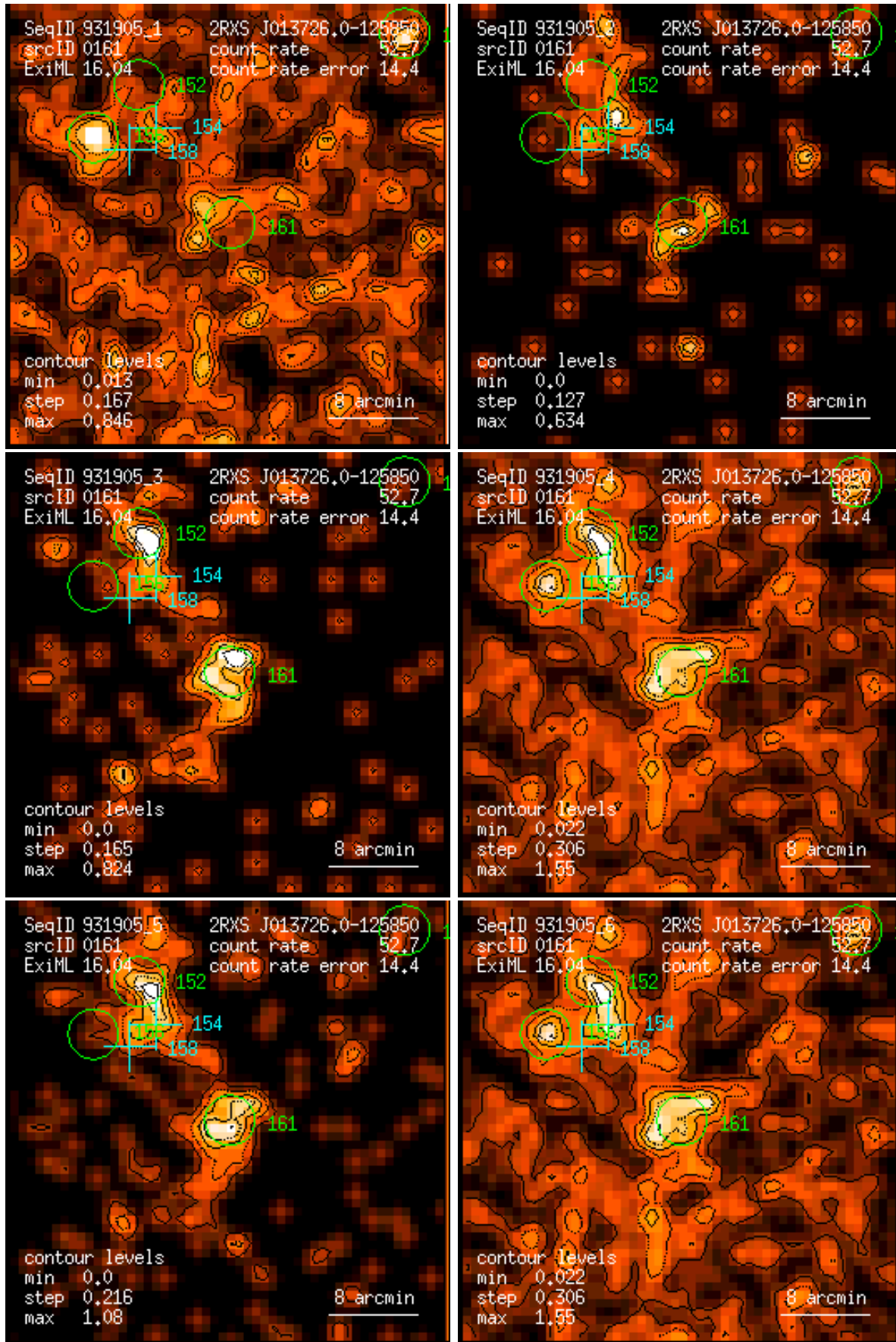
Figure 161: RASS 931905: detection 0161: band rate images, Gaussian filter: (1) PSPC channels 11 – 41, (2) 52 – 90, (3) 91 – 201, (4) 11 – 235, (5) 52 – 201, (6) 11 – 201. Broad band rates in counts/ks. Band rate contour levels in counts/ks/arcmin 2 .
