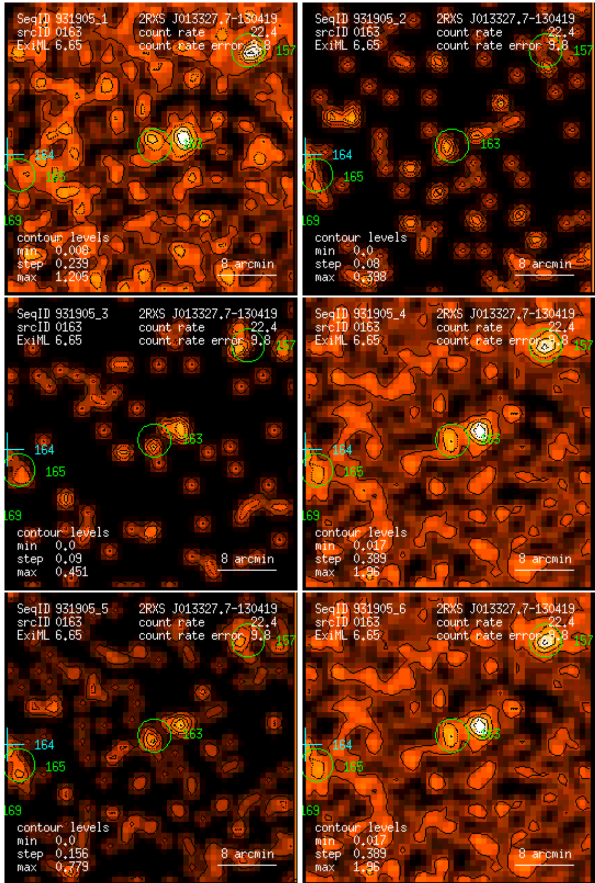
Figure 163: RASS 931905: detection 0163: band rate images, Gaussian filter: (1) PSPC channels 11 – 41, (2) 52 – 90, (3) 91 – 201, (4) 11 – 235, (5) 52 – 201, (6) 11 – 201. Broad band rates in counts/ks. Band rate contour levels in counts/ks/arcmin 2 .
