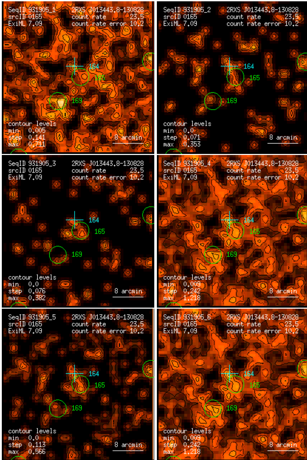
Figure 165: RASS 931905: detection 0165: band rate images, Gaussian filter: (1) PSPC channels 11 – 41, (2) 52 – 90, (3) 91 – 201, (4) 11 – 235, (5) 52 – 201, (6) 11 – 201. Broad band rates in counts/ks. Band rate contour levels in counts/ks/arcmin 2 .
