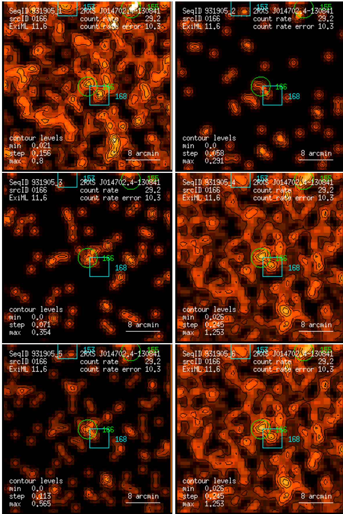
Figure 166: RASS 931905: detection 0166: band rate images, Gaussian filter: (1) PSPC channels 11 – 41, (2) 52 – 90, (3) 91 – 201, (4) 11 – 235, (5) 52 – 201, (6) 11 – 201. Broad band rates in counts/ks. Band rate contour levels in counts/ks/arcmin 2 .
