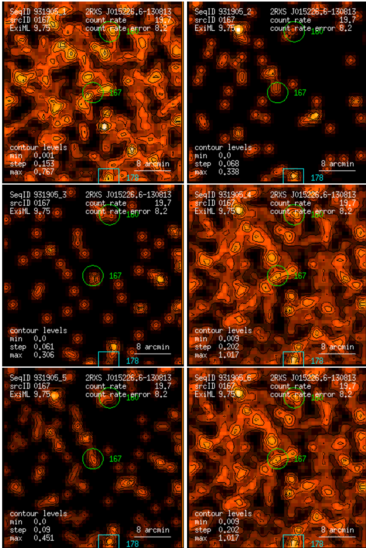
Figure 167: RASS 931905: detection 0167: band rate images, Gaussian filter: (1) PSPC channels 11 – 41, (2) 52 – 90, (3) 91 – 201, (4) 11 – 235, (5) 52 – 201, (6) 11 – 201. Broad band rates in counts/ks. Band rate contour levels in counts/ks/arcmin 2 .
