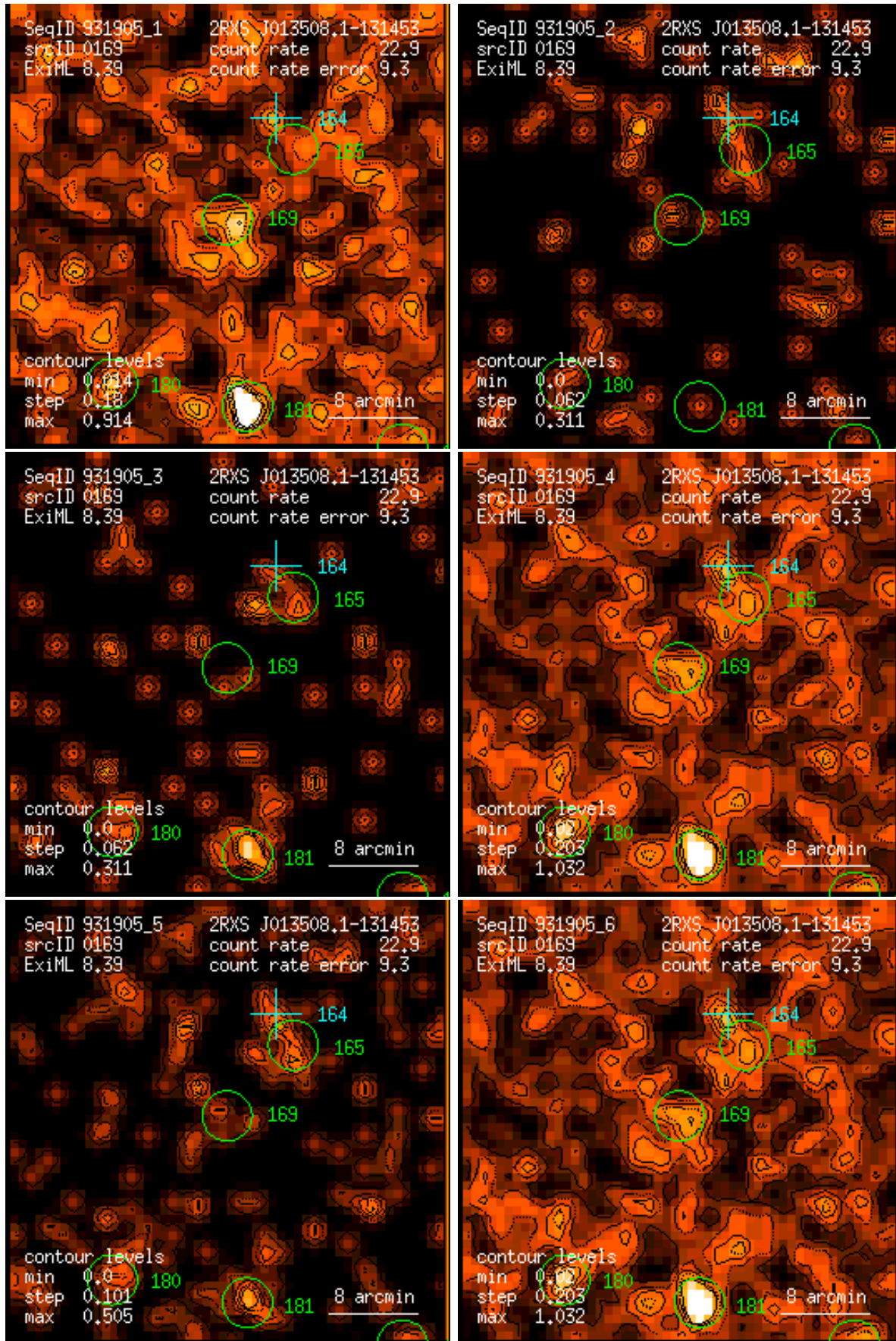
Figure 169: RASS 931905: detection 0169: band rate images, Gaussian filter: (1) PSPC channels 11 – 41, (2) 52 – 90, (3) 91 – 201, (4) 11 – 235, (5) 52 – 201, (6) 11 – 201. Broad band rates in counts/ks. Band rate contour levels in counts/ks/arcmin 2 .
