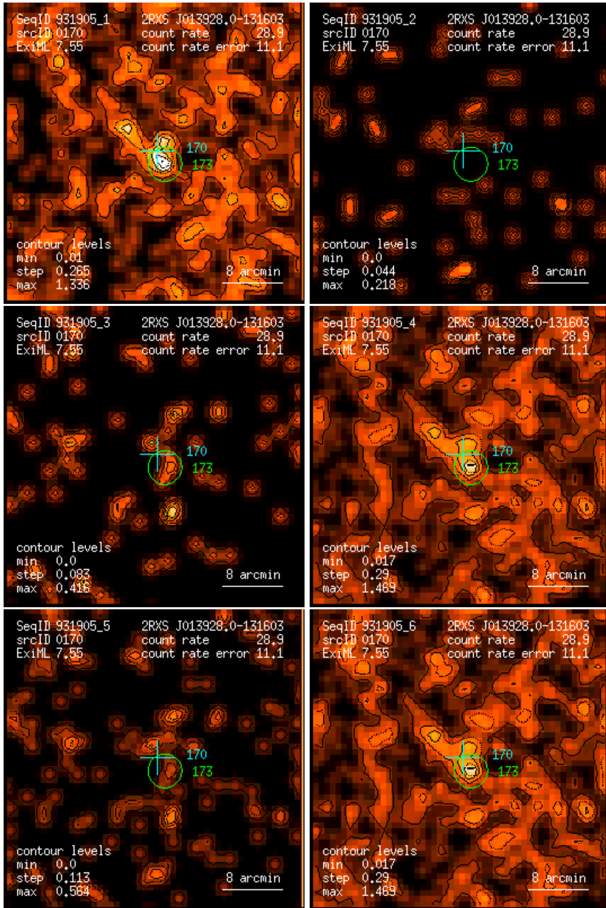
Figure 170: RASS 931905: detection 0170: band rate images, Gaussian filter: (1) PSPC channels 11 – 41, (2) 52 – 90, (3) 91 – 201, (4) 11 – 235, (5) 52 – 201, (6) 11 – 201. Broad band rates in counts/ks. Band rate contour levels in counts/ks/arcmin 2 .
