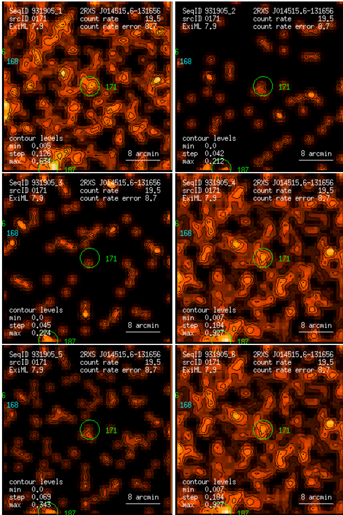
Figure 171: RASS 931905: detection 0171: band rate images, Gaussian filter: (1) PSPC channels 11 – 41, (2) 52 – 90, (3) 91 – 201, (4) 11 – 235, (5) 52 – 201, (6) 11 – 201. Broad band rates in counts/ks. Band rate contour levels in counts/ks/arcmin 2 .
