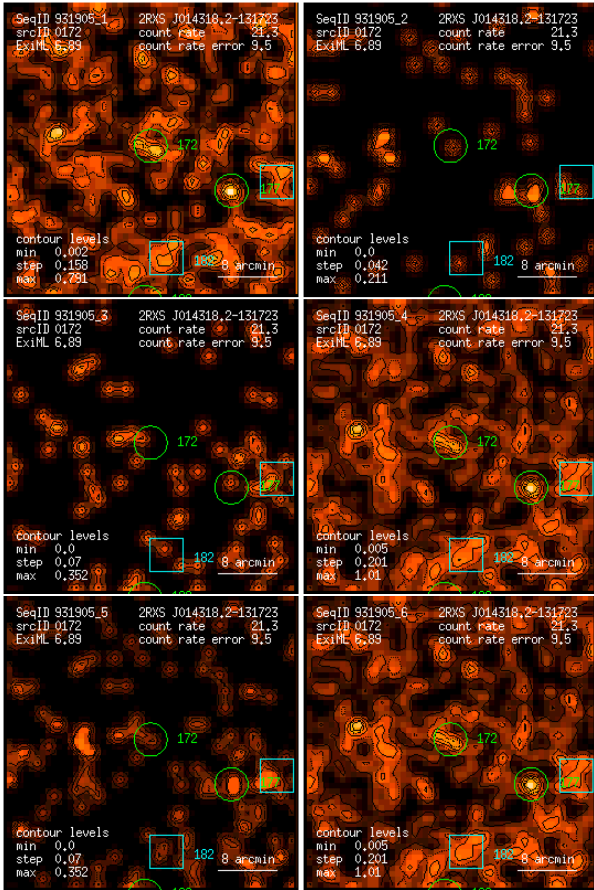
Figure 172: RASS 931905: detection 0172: band rate images, Gaussian filter: (1) PSPC channels 11 – 41, (2) 52 – 90, (3) 91 – 201, (4) 11 – 235, (5) 52 – 201, (6) 11 – 201. Broad band rates in counts/ks. Band rate contour levels in counts/ks/arcmin 2 .
