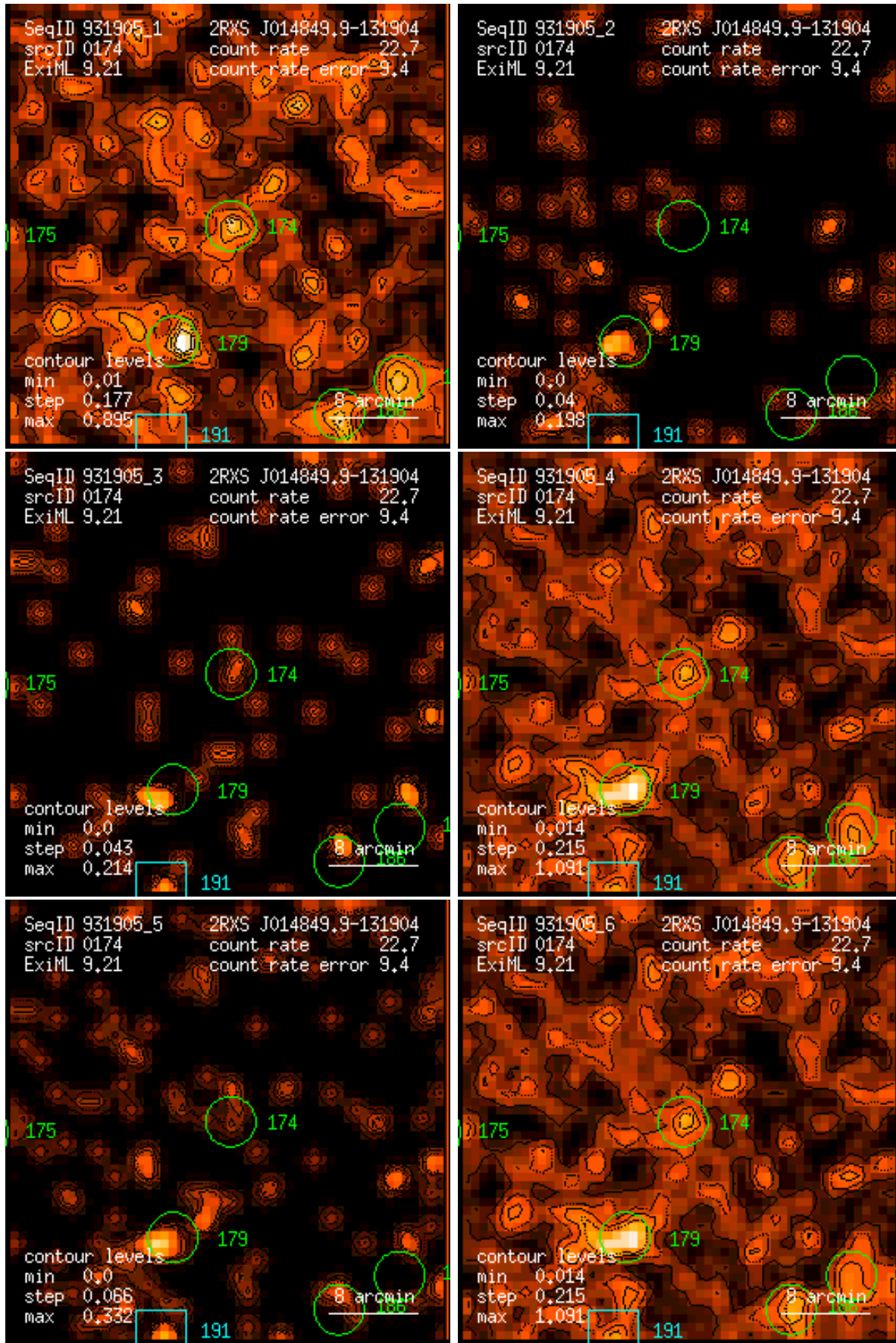
Figure 174: RASS 931905: detection 0174: band rate images, Gaussian filter: (1) PSPC channels 11 – 41, (2) 52 – 90, (3) 91 – 201, (4) 11 – 235, (5) 52 – 201, (6) 11 – 201. Broad band rates in counts/ks. Band rate contour levels in counts/ks/arcmin 2 .
