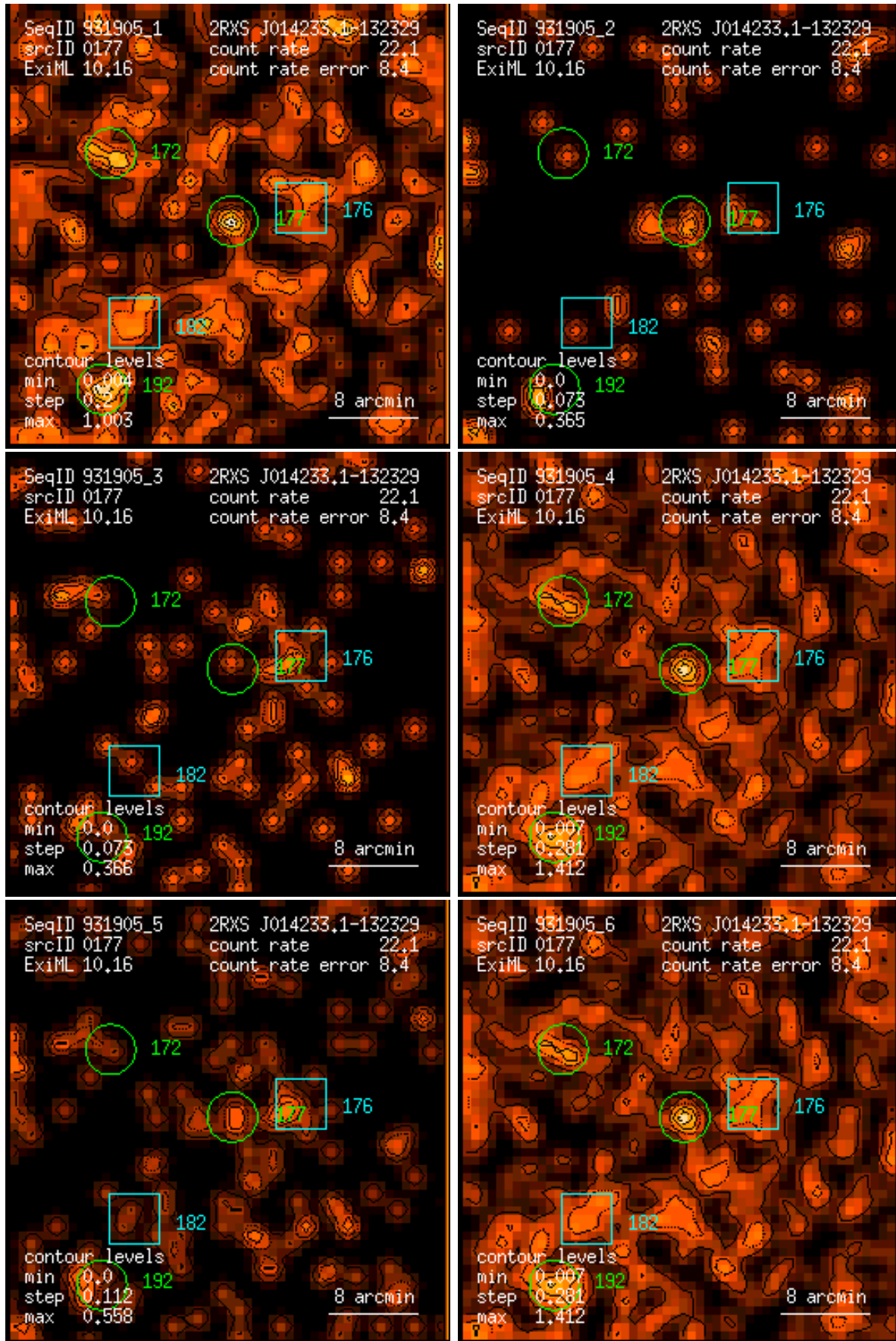
Figure 177: RASS 931905: detection 0177: band rate images, Gaussian filter: (1) PSPC channels 11 – 41, (2) 52 – 90, (3) 91 – 201, (4) 11 – 235, (5) 52 – 201, (6) 11 – 201. Broad band rates in counts/ks. Band rate contour levels in counts/ks/arcmin 2 .
