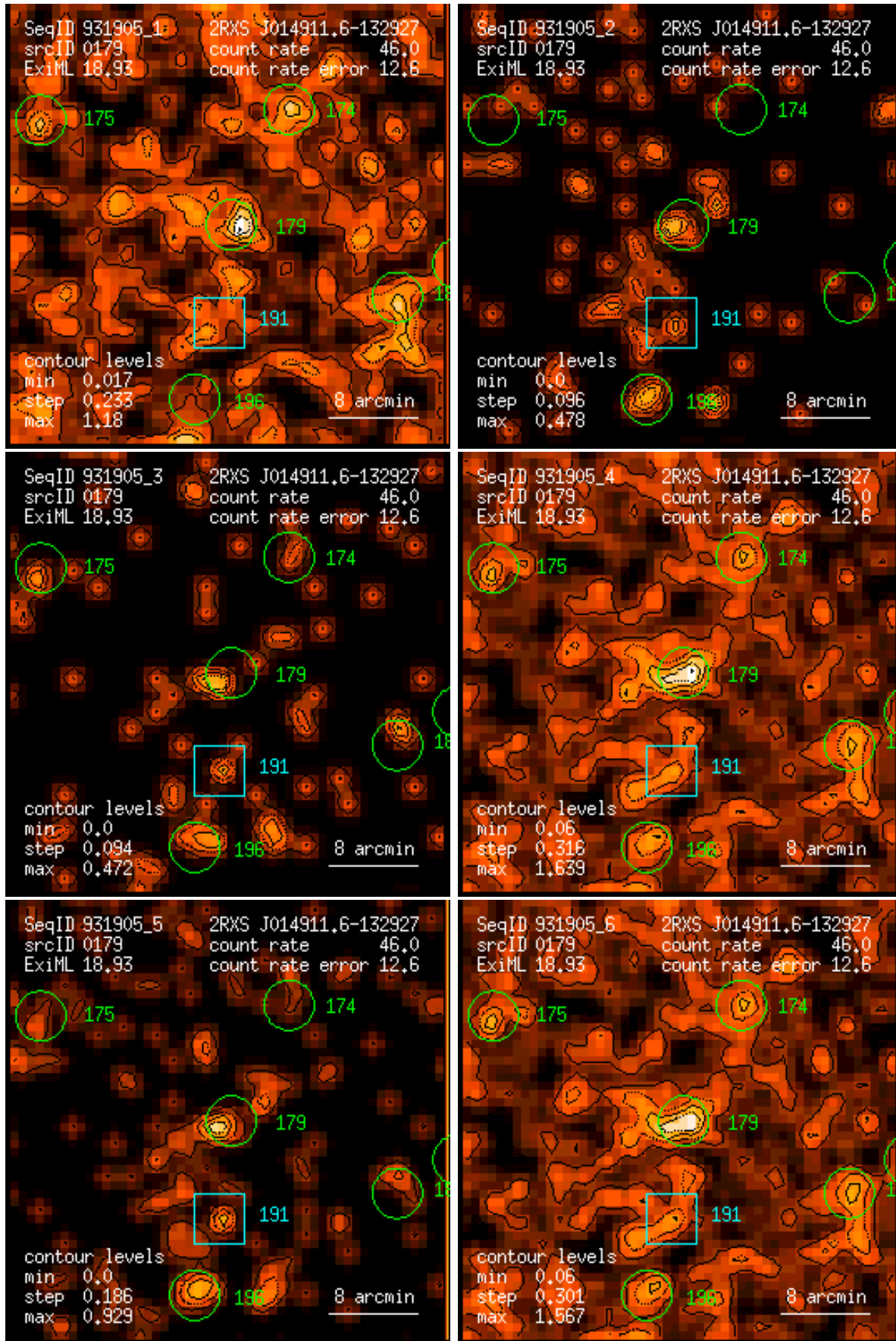
Figure 179: RASS 931905: detection 0179: band rate images, Gaussian filter: (1) PSPC channels 11 – 41, (2) 52 – 90, (3) 91 – 201, (4) 11 – 235, (5) 52 – 201, (6) 11 – 201. Broad band rates in counts/ks. Band rate contour levels in counts/ks/arcmin 2 .
