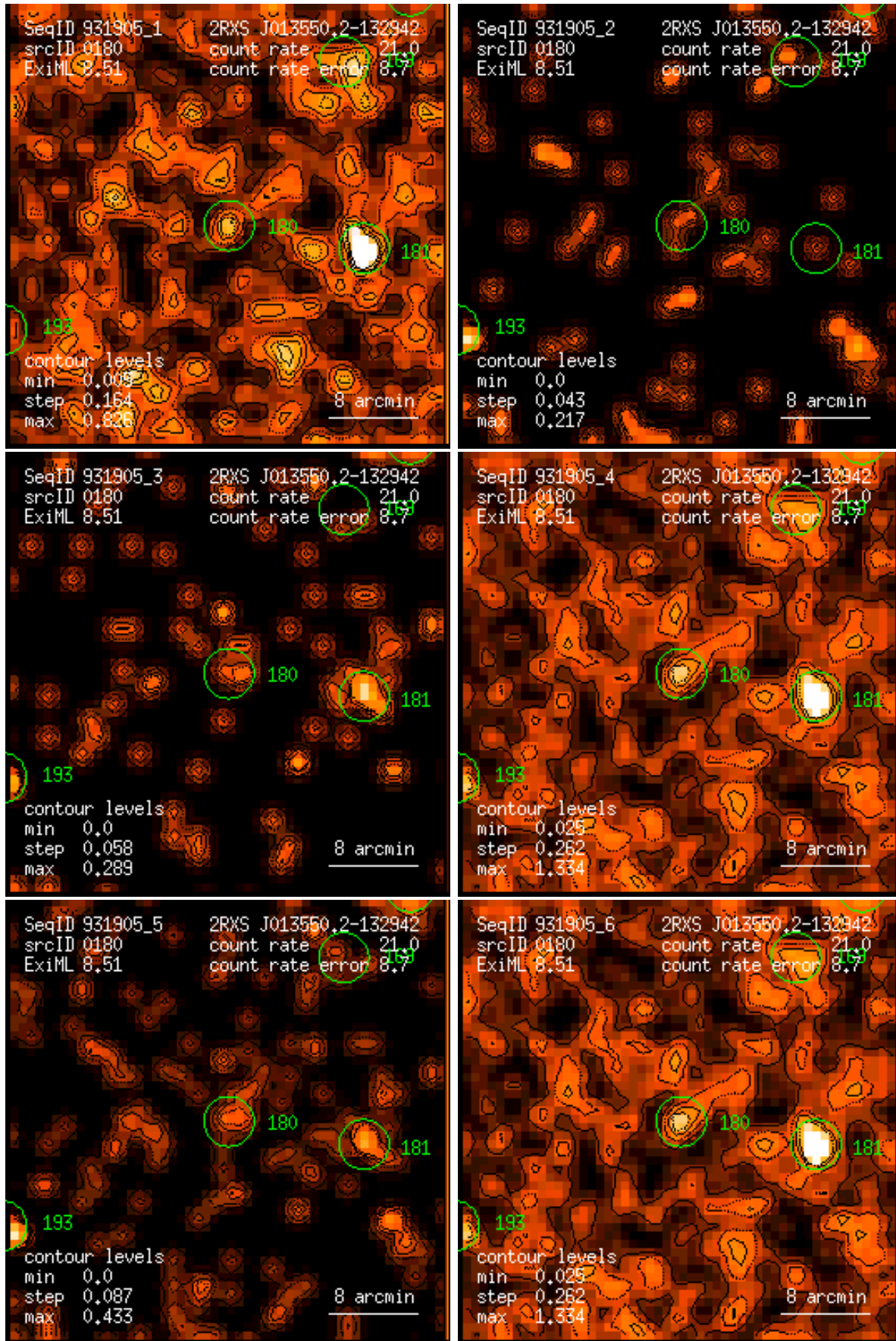
Figure 180: RASS 931905: detection 0180: band rate images, Gaussian filter: (1) PSPC channels 11 – 41, (2) 52 – 90, (3) 91 – 201, (4) 11 – 235, (5) 52 – 201, (6) 11 – 201. Broad band rates in counts/ks. Band rate contour levels in counts/ks/arcmin 2 .
