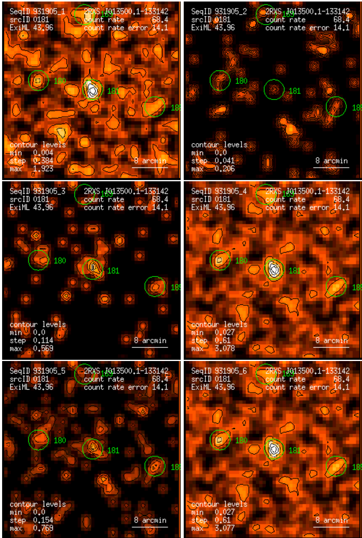
Figure 181: RASS 931905: detection 0181: band rate images, Gaussian filter: (1) PSPC channels 11 – 41, (2) 52 – 90, (3) 91 – 201, (4) 11 – 235, (5) 52 – 201, (6) 11 – 201. Broad band rates in counts/ks. Band rate contour levels in counts/ks/arcmin 2 .
