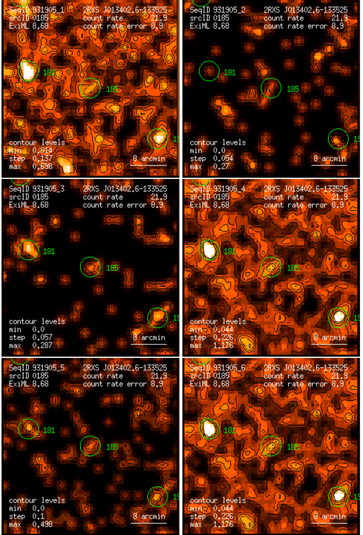
Figure 185: RASS 931905: detection 0185: band rate images, Gaussian filter: (1) PSPC channels 11 – 41, (2) 52 – 90, (3) 91 – 201, (4) 11 – 235, (5) 52 – 201, (6) 11 – 201. Broad band rates in counts/ks. Band rate contour levels in counts/ks/arcmin 2 .
