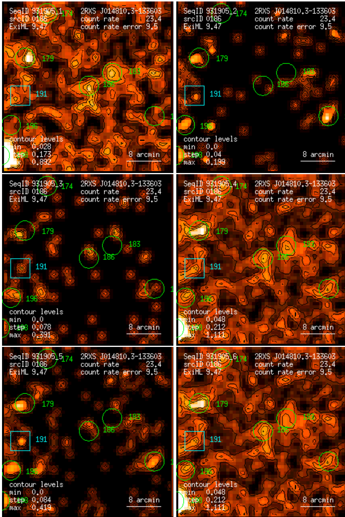
Figure 186: RASS 931905: detection 0186: band rate images, Gaussian filter: (1) PSPC channels 11 – 41, (2) 52 – 90, (3) 91 – 201, (4) 11 – 235, (5) 52 – 201, (6) 11 – 201. Broad band rates in counts/ks. Band rate contour levels in counts/ks/arcmin 2 .
