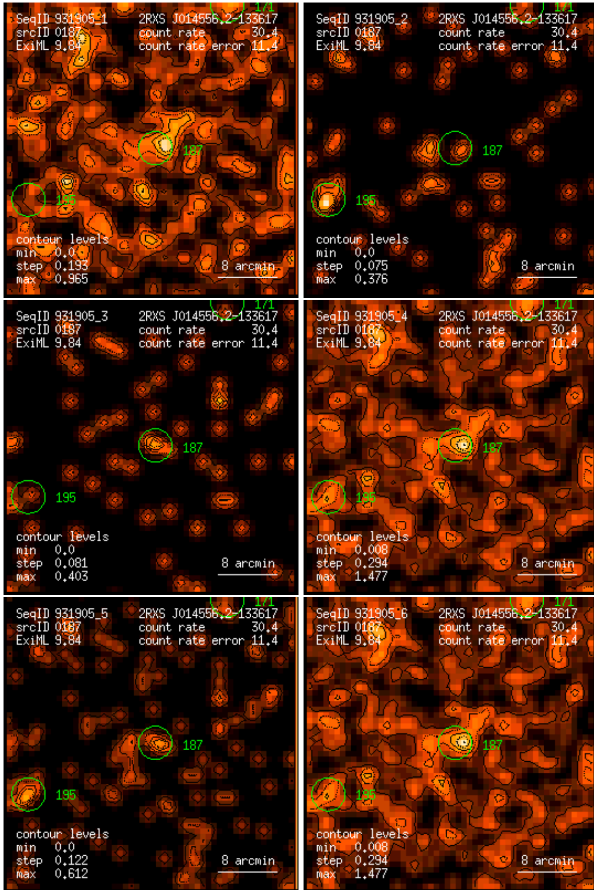
Figure 187: RASS 931905: detection 0187: band rate images, Gaussian filter: (1) PSPC channels 11 – 41, (2) 52 – 90, (3) 91 – 201, (4) 11 – 235, (5) 52 – 201, (6) 11 – 201. Broad band rates in counts/ks. Band rate contour levels in counts/ks/arcmin 2 .
