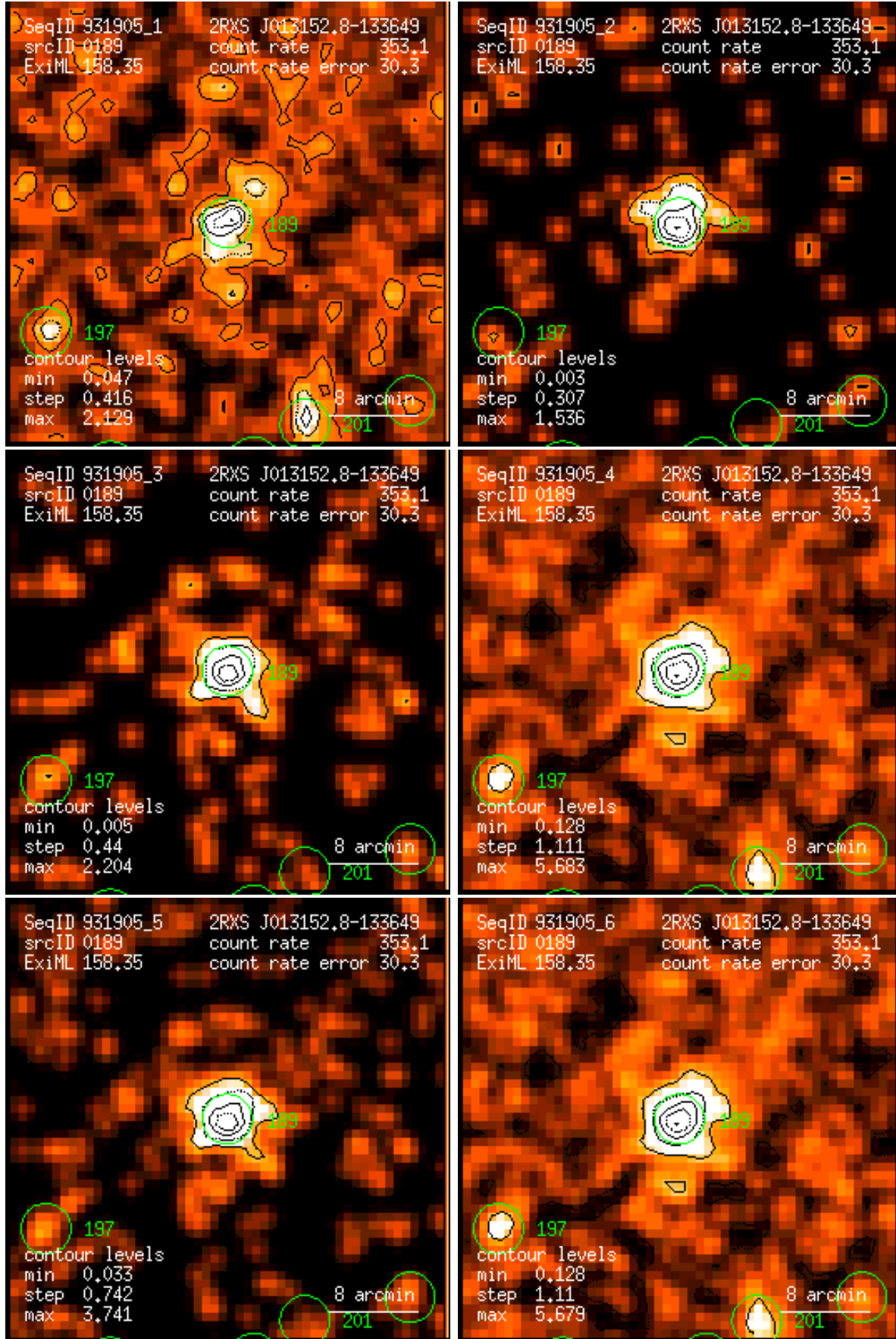
Figure 189: RASS 931905: detection 0189: band rate images, Gaussian filter: (1) PSPC channels 11 – 41, (2) 52 – 90, (3) 91 – 201, (4) 11 – 235, (5) 52 – 201, (6) 11 – 201. Broad band rates in counts/ks. Band rate contour levels in counts/ks/arcmin 2 .
