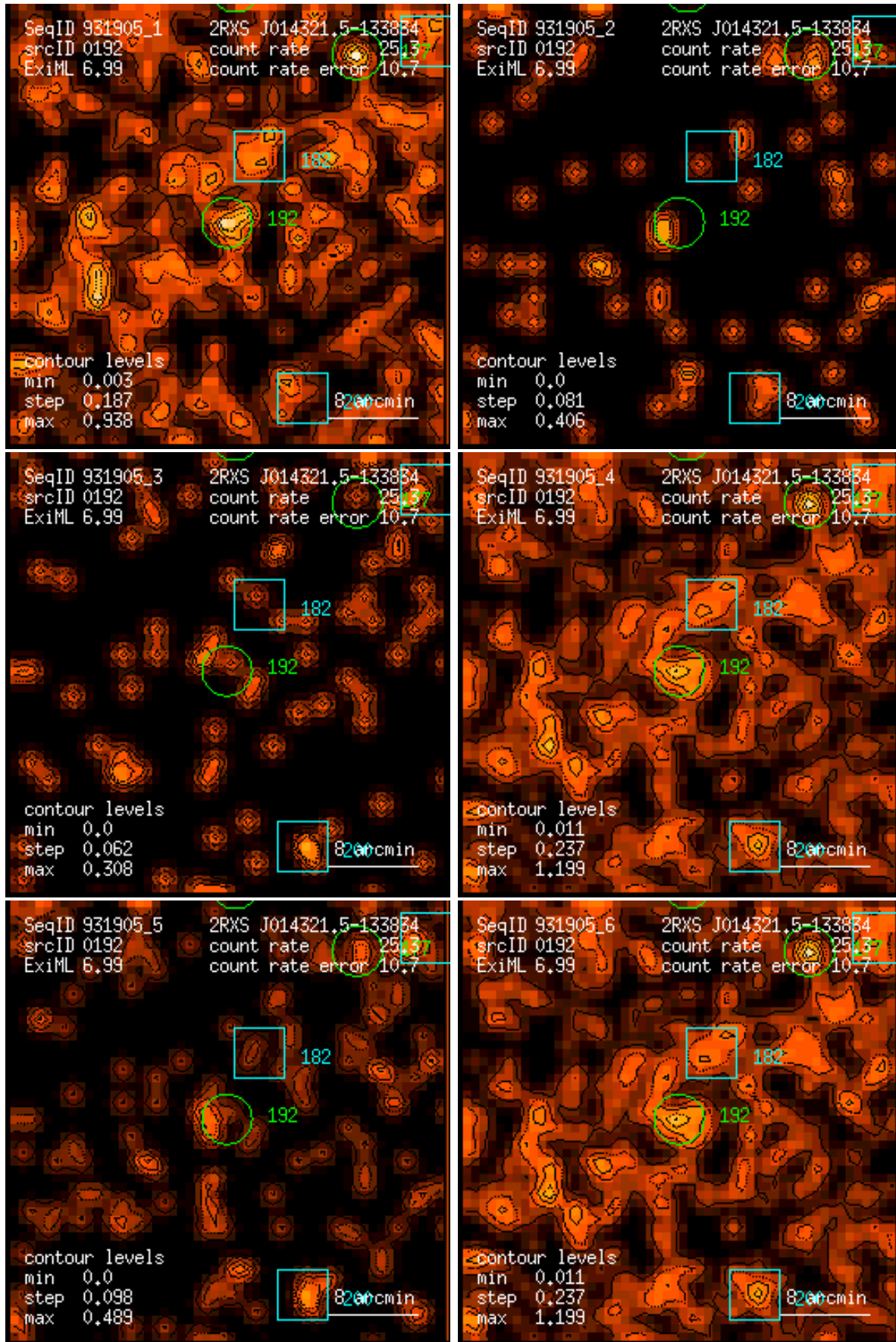
Figure 192: RASS 931905: detection 0192: band rate images, Gaussian filter: (1) PSPC channels 11 – 41, (2) 52 – 90, (3) 91 – 201, (4) 11 – 235, (5) 52 – 201, (6) 11 – 201. Broad band rates in counts/ks. Band rate contour levels in counts/ks/arcmin 2 .
