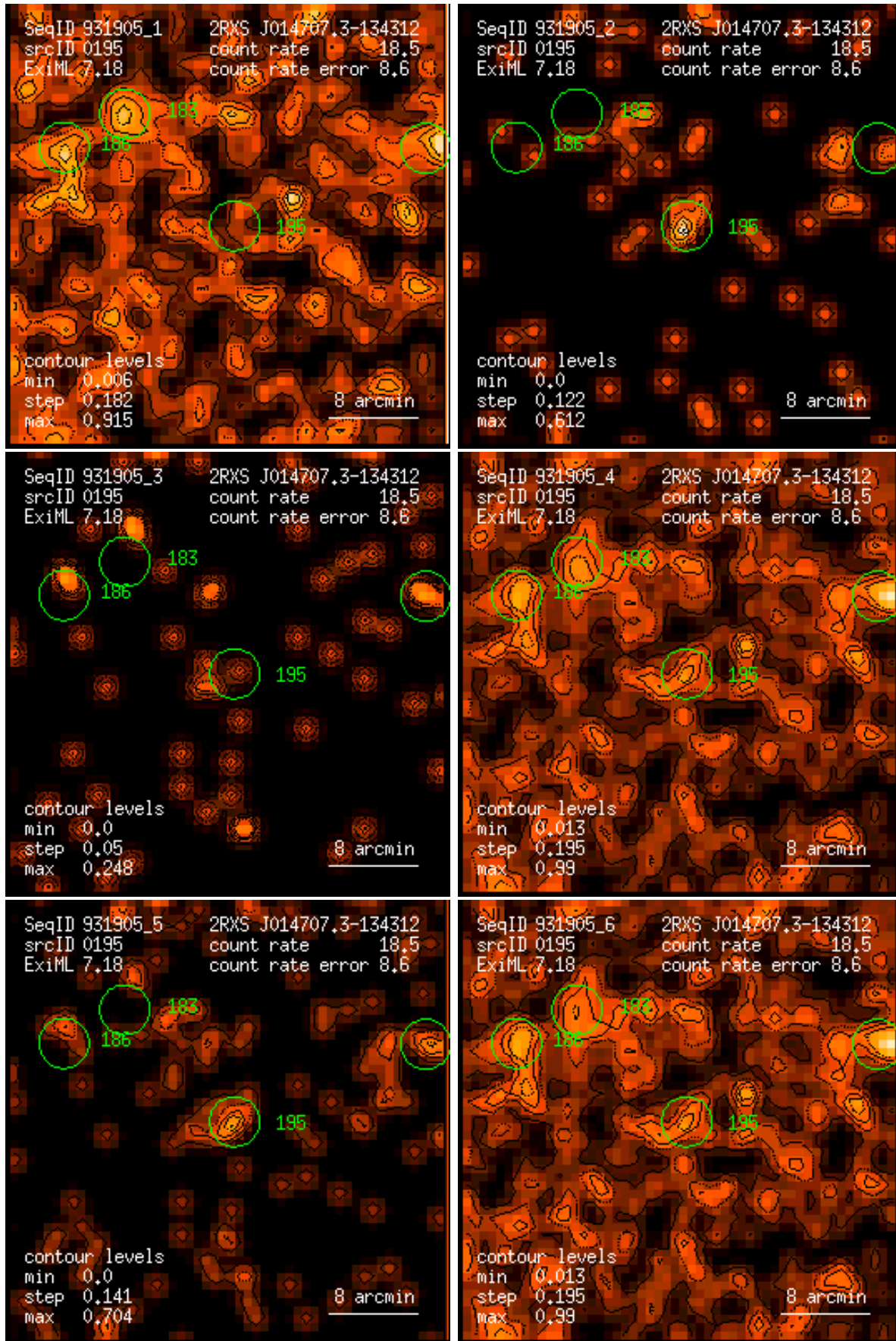
Figure 195: RASS 931905: detection 0195: band rate images, Gaussian filter: (1) PSPC channels 11 – 41, (2) 52 – 90, (3) 91 – 201, (4) 11 – 235, (5) 52 – 201, (6) 11 – 201. Broad band rates in counts/ks. Band rate contour levels in counts/ks/arcmin 2 .
