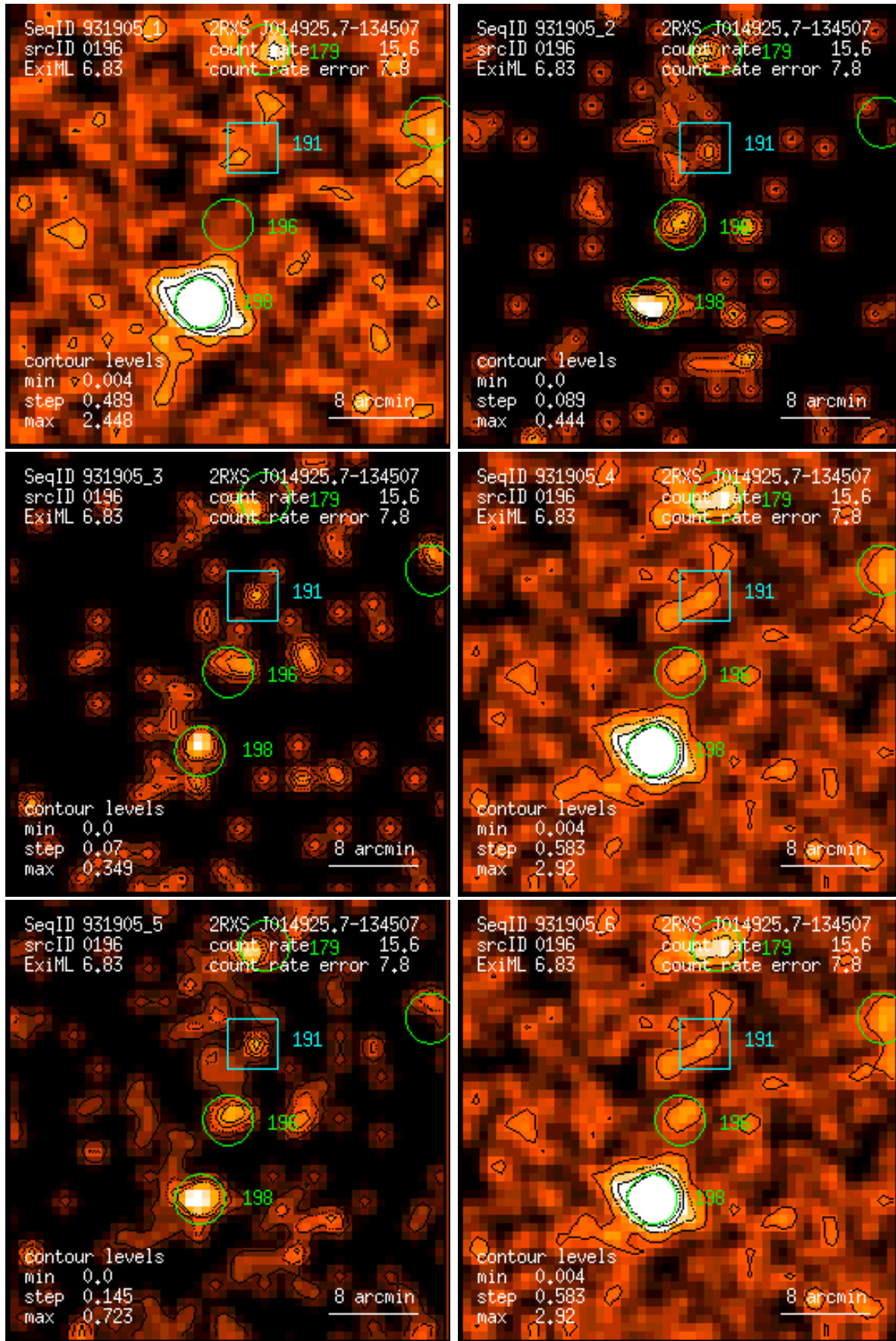
Figure 196: RASS 931905: detection 0196: band rate images, Gaussian filter: (1) PSPC channels 11 – 41, (2) 52 – 90, (3) 91 – 201, (4) 11 – 235, (5) 52 – 201, (6) 11 – 201. Broad band rates in counts/ks. Band rate contour levels in counts/ks/arcmin 2 .
