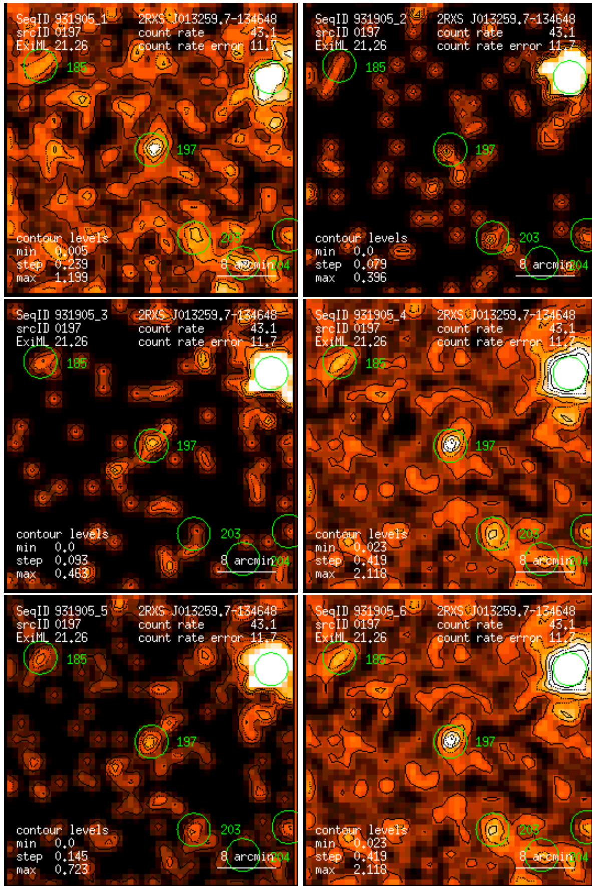
Figure 197: RASS 931905: detection 0197: band rate images, Gaussian filter: (1) PSPC channels 11 – 41, (2) 52 – 90, (3) 91 – 201, (4) 11 – 235, (5) 52 – 201, (6) 11 – 201. Broad band rates in counts/ks. Band rate contour levels in counts/ks/arcmin 2 .
