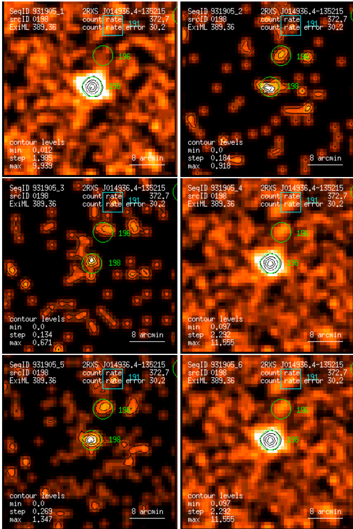
Figure 198: RASS 931905: detection 0198: band rate images, Gaussian filter: (1) PSPP channels 11 – 41, (2) 52 – 90, (3) 91 – 201, (4) 11 – 235, (5) 52 – 201, (6) 11 – 201. Broad band rates in counts/ks. Band rate contour levels in counts/ks/arcmin 2 .
