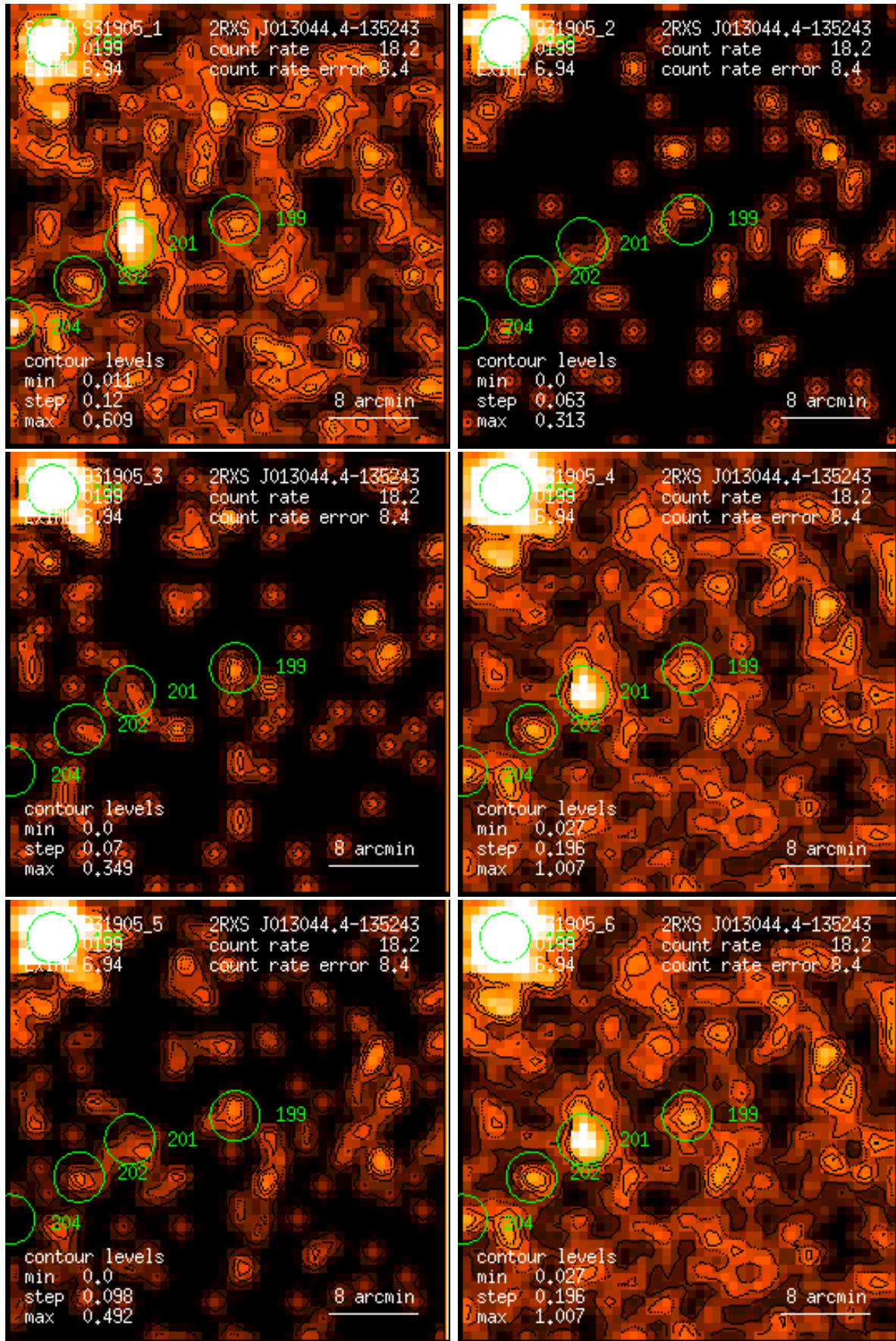
Figure 199: RASS 931905: detection 0199: band rate images, Gaussian filter: (1) PSPC channels 11 – 41, (2) 52 – 90, (3) 91 – 201, (4) 11 – 235, (5) 52 – 201, (6) 11 – 201. Broad band rates in counts/ks. Band rate contour levels in counts/ks/arcmin 2 .
