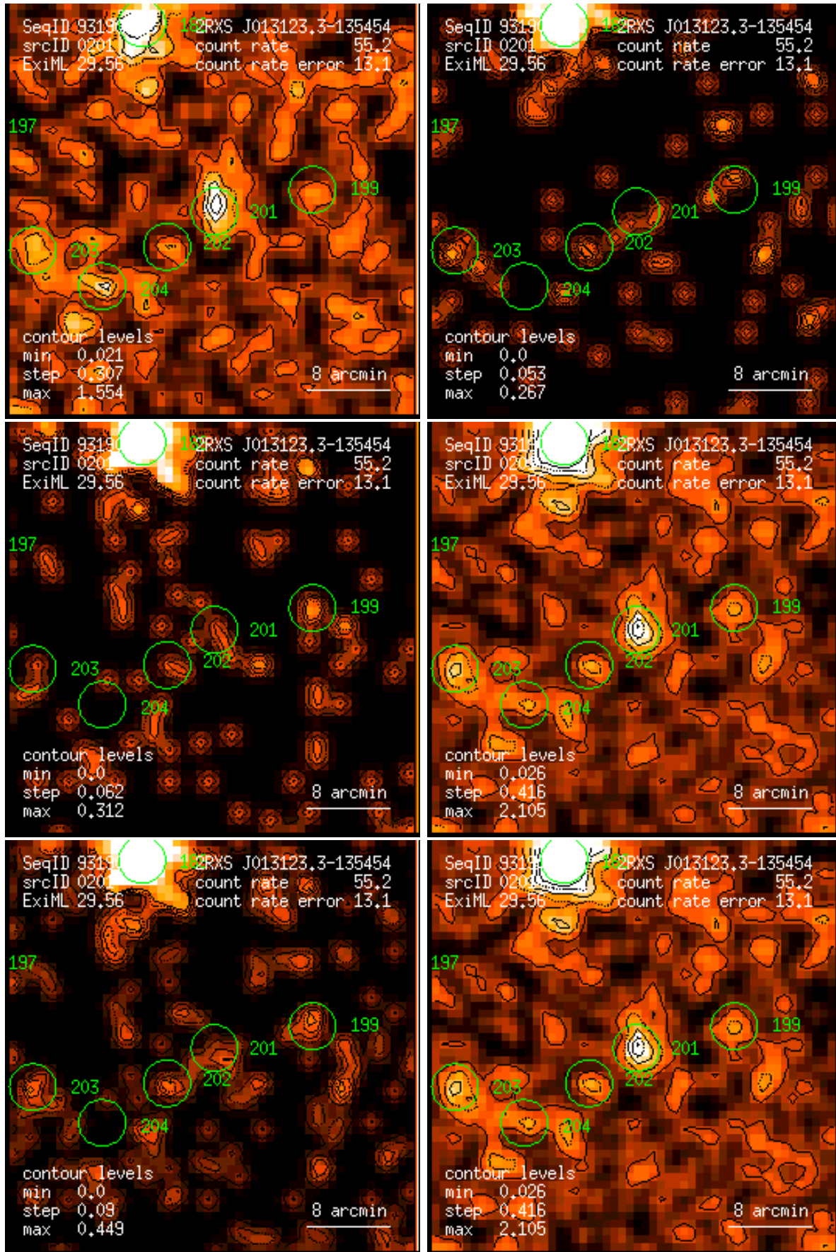
Figure 201: RASS 931905: detection 0201: band rate images, Gaussian filter: (1) PSPC channels 11 – 41, (2) 52 – 90, (3) 91 – 201, (4) 11 – 235, (5) 52 – 201, (6) 11 – 201. Broad band rates in counts/ks. Band rate contour levels in counts/ks/arcmin 2 .
