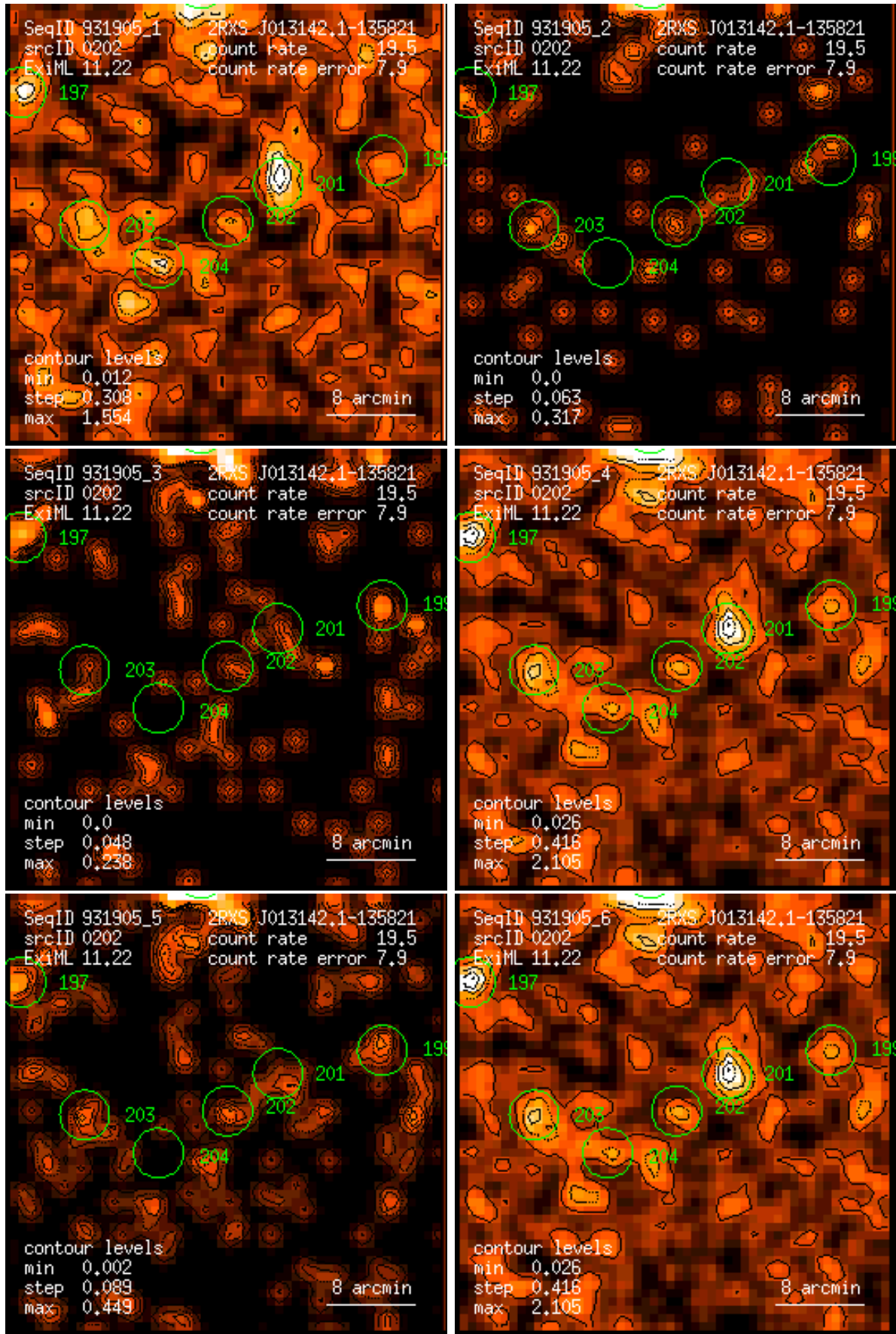
Figure 202: RASS 931905: detection 0202: band rate images, Gaussian filter: (1) PSPC channels 11 – 41, (2) 52 – 90, (3) 91 – 201, (4) 11 – 235, (5) 52 – 201, (6) 11 – 201. Broad band rates in counts/ks. Band rate contour levels in counts/ks/arcmin 2 .
