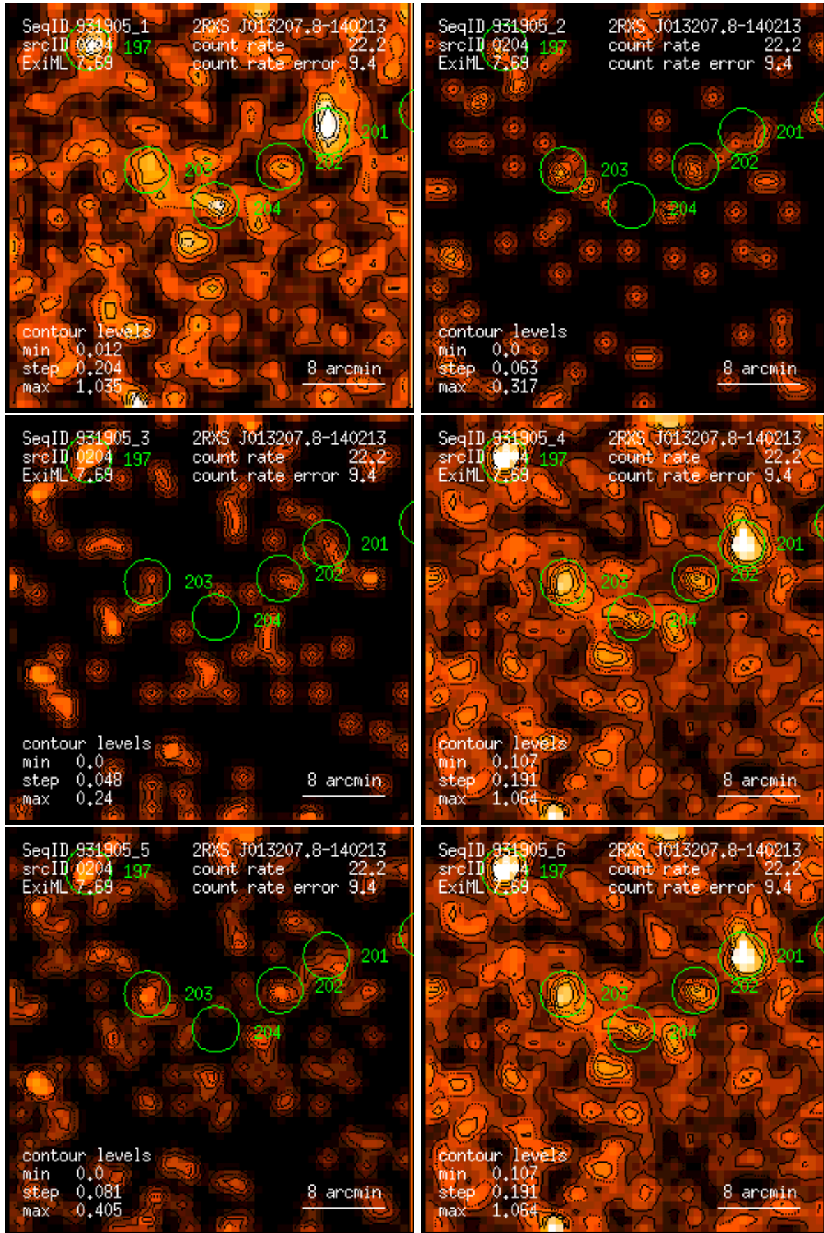
Figure 204: RASS 931905: detection 0204: band rate images, Gaussian filter: (1) PSPC channels 11 – 41, (2) 52 – 90, (3) 91 – 201, (4) 11 – 235, (5) 52 – 201, (6) 11 – 201. Broad band rates in counts/ks. Band rate contour levels in counts/ks/arcmin 2 .
