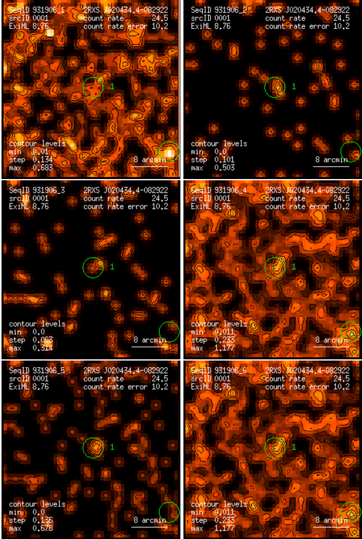
Figure 1: RASS 931906: detection 0001: band rate images, Gaussian filter: (1) PSPC channels 11 – 41, (2) 52 – 90, (3) 91 – 201, (4) 11 – 235, (5) 52 – 201, (6) 11 – 201. Broad band rates in counts/ks. Band rate contour levels in counts/ks/arcmin 2 .
