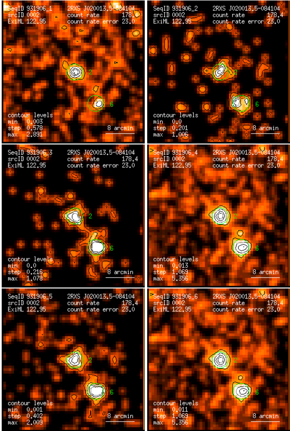
Figure 2: RASS 931906: detection 0002: band rate images, Gaussian filter: (1) PSPC channels 11 – 41, (2) 52 – 90, (3) 91 – 201, (4) 11 – 235, (5) 52 – 201, (6) 11 – 201. Broad band rates in counts/ks. Band rate contour levels in counts/ks/arcmin 2 .
