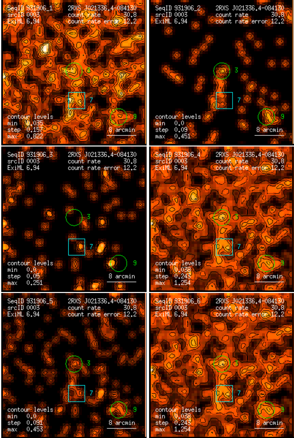
Figure 3: RASS 931906: detection 0003: band rate images, Gaussian filter: (1) PSPC channels 11 – 41, (2) 52 – 90, (3) 91 – 201, (4) 11 – 235, (5) 52 – 201, (6) 11 – 201. Broad band rates in counts/ks. Band rate contour levels in counts/ks/arcmin 2 .
