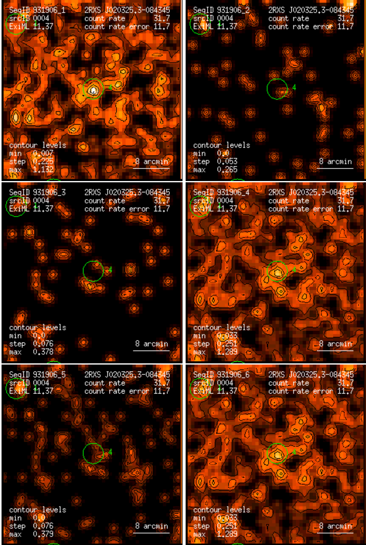
Figure 4: RASS 931906: detection 0004: band rate images, Gaussian filter: (1) PSPC channels 11 – 41, (2) 52 – 90, (3) 91 – 201, (4) 11 – 235, (5) 52 – 201, (6) 11 – 201. Broad band rates in counts/ks. Band rate contour levels in counts/ks/arcmin 2 .
