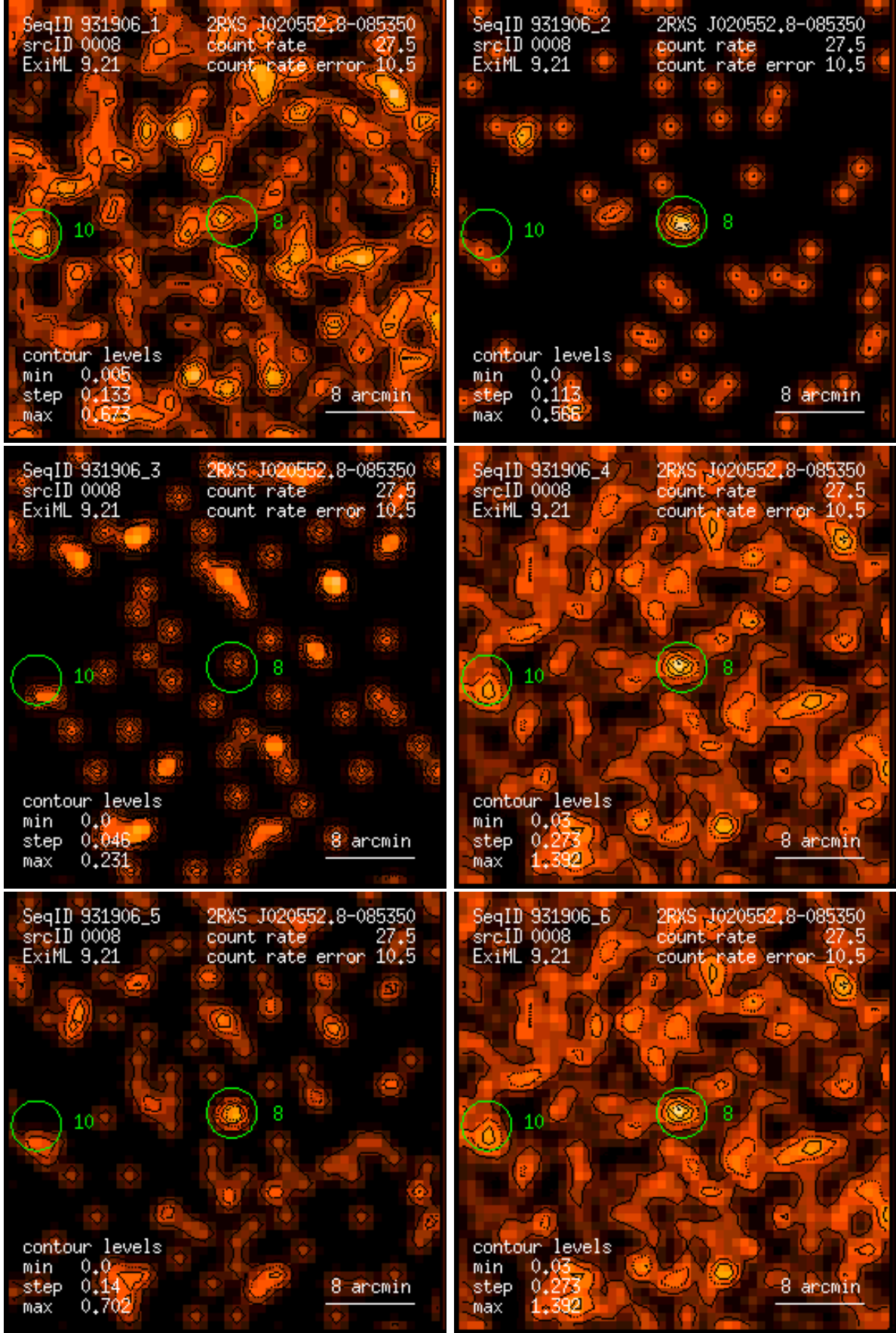
Figure 8: RASS 931906: detection 0008: band rate images, Gaussian filter: (1) PSPC channels 11 – 41, (2) 52 – 90, (3) 91 – 201, (4) 11 – 235, (5) 52 – 201, (6) 11 – 201. Broad band rates in counts/ks. Band rate contour levels in counts/ks/arcmin 2 .
