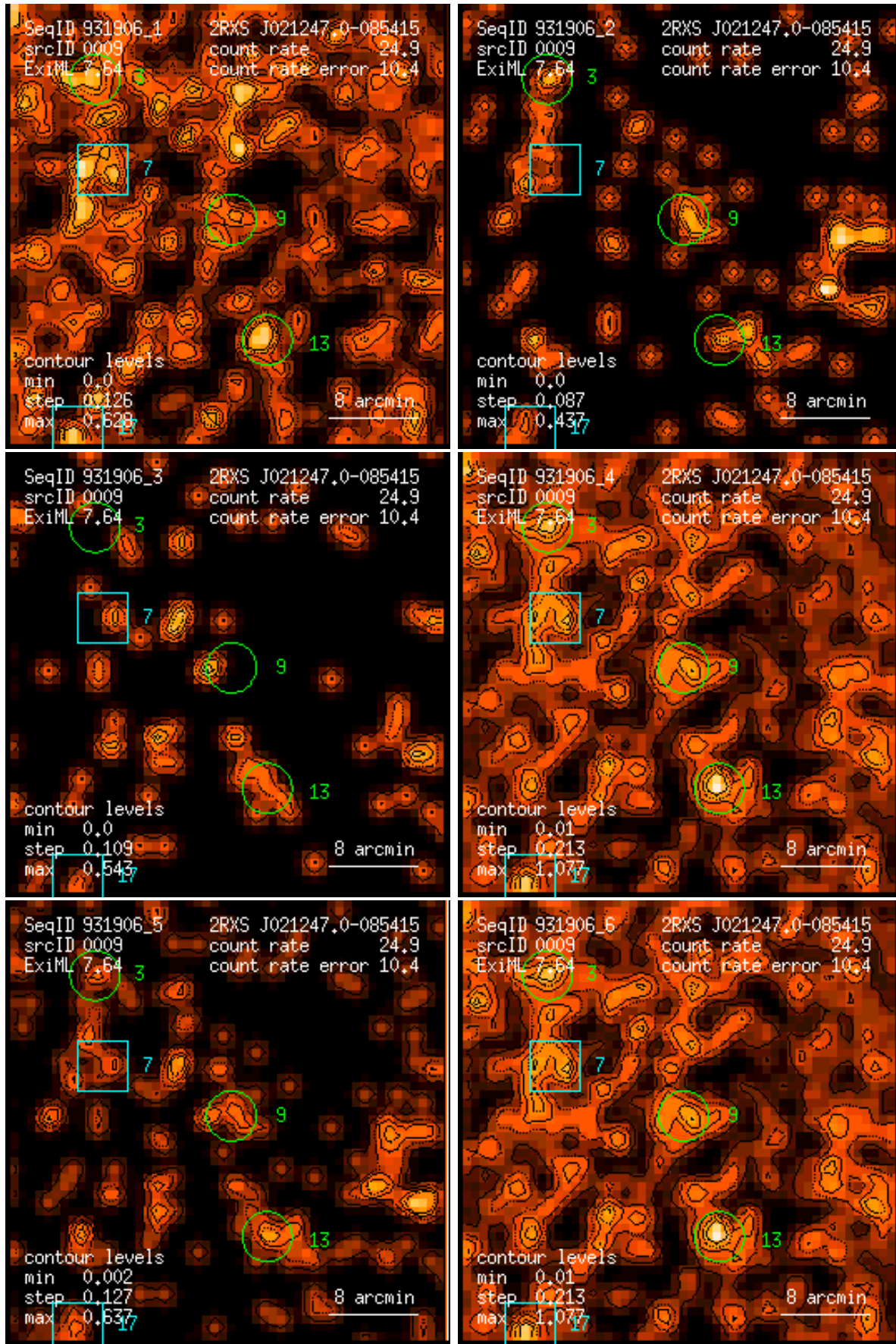
Figure 9: RASS 931906: detection 0009: band rate images, Gaussian filter: (1) PSPC channels 11 – 41, (2) 52 – 90, (3) 91 – 201, (4) 11 – 235, (5) 52 – 201, (6) 11 – 201. Broad band rates in counts/ks. Band rate contour levels in counts/ks/arcmin 2 .
