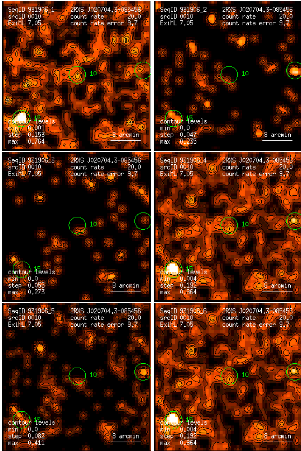
Figure 10: RASS 931906: detection 0010: band rate images, Gaussian filter: (1) PSPC channels 11 – 41, (2) 52 – 90, (3) 91 – 201, (4) 11 – 235, (5) 52 – 201, (6) 11 – 201. Broad band rates in counts/ks. Band rate contour levels in counts/ks/arcmin 2 .
