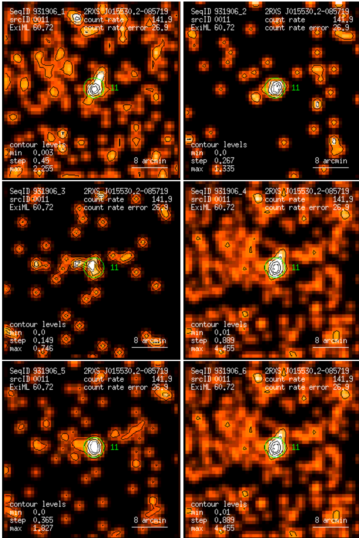
Figure 11: RASS 931906: detection 0011: band rate images, Gaussian filter: (1) PSPC channels 11 – 41, (2) 52 – 90, (3) 91 – 201, (4) 11 – 235, (5) 52 – 201, (6) 11 – 201. Broad band rates in counts/ks. Band rate contour levels in counts/ks/arcmin 2 .
