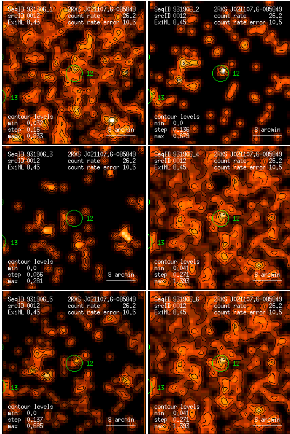
Figure 12: RASS 931906: detection 0012: band rate images, Gaussian filter: (1) PSPC channels 11 – 41, (2) 52 – 90, (3) 91 – 201, (4) 11 – 235, (5) 52 – 201, (6) 11 – 201. Broad band rates in counts/ks. Band rate contour levels in counts/ks/arcmin 2 .
