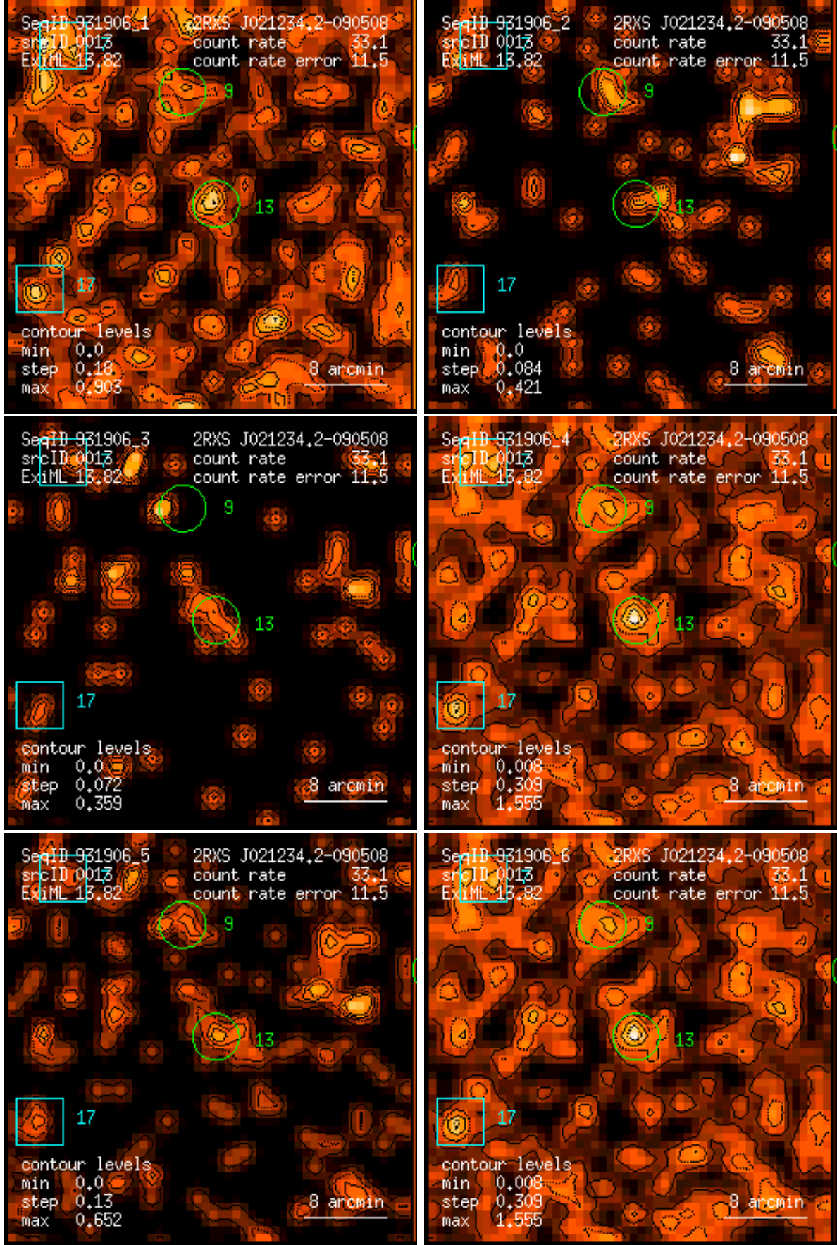
Figure 13: RASS 931906: detection 0013: band rate images, Gaussian filter: (1) PSPC channels 11 – 41, (2) 52 – 90, (3) 91 – 201, (4) 11 – 235, (5) 52 – 201, (6) 11 – 201. Broad band rates in counts/ks. Band rate contour levels in counts/ks/arcmin 2 .
