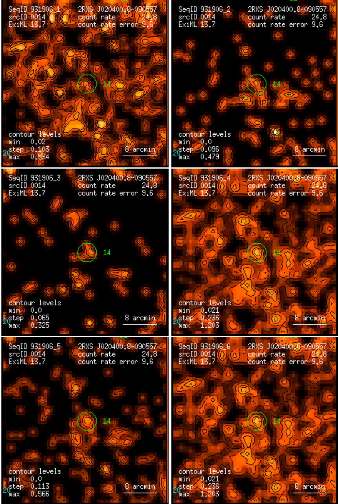
Figure 14: RASS 931906: detection 0014: band rate images, Gaussian filter: (1) PSPC channels 11 – 41, (2) 52 – 90, (3) 91 – 201, (4) 11 – 235, (5) 52 – 201, (6) 11 – 201. Broad band rates in counts/ks. Band rate contour levels in counts/ks/arcmin 2 .
