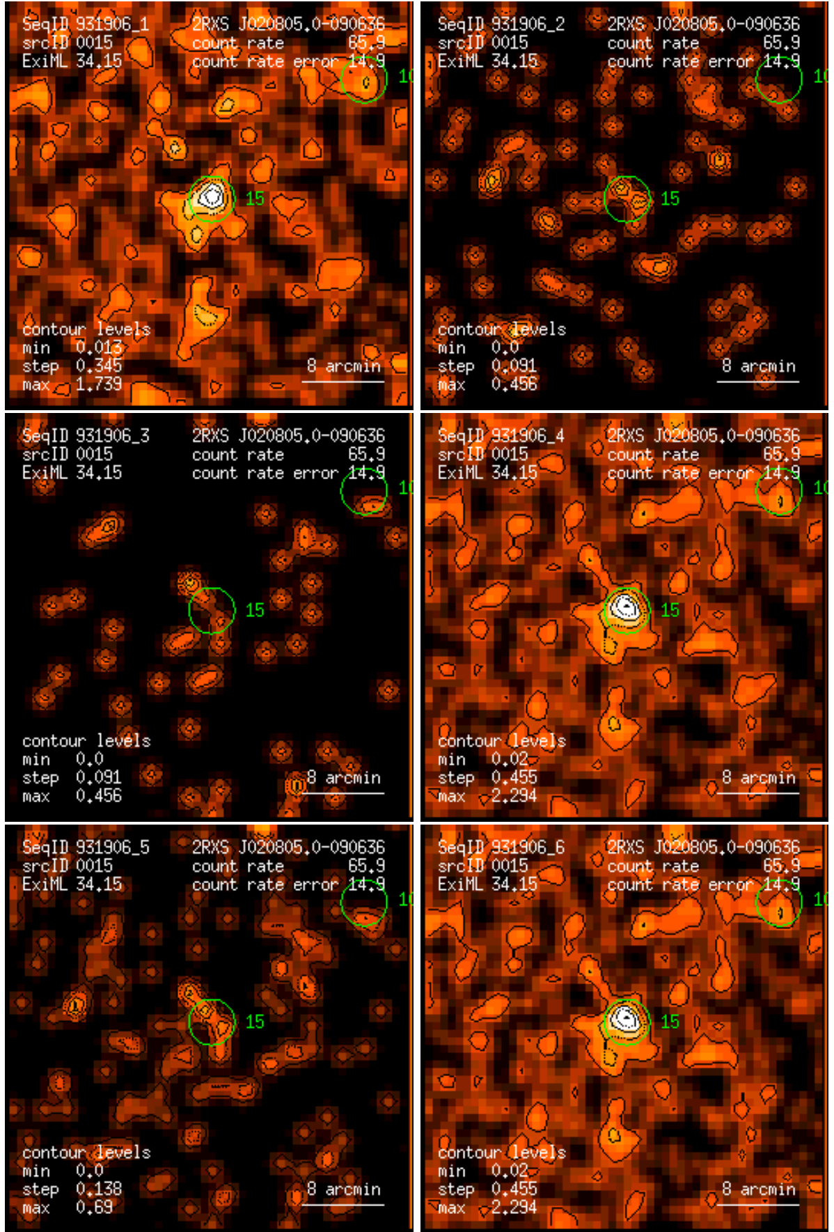
Figure 15: RASS 931906: detection 0015: band rate images, Gaussian filter: (1) PSPC channels 11 – 41, (2) 52 – 90, (3) 91 – 201, (4) 11 – 235, (5) 52 – 201, (6) 11 – 201. Broad band rates in counts/ks. Band rate contour levels in counts/ks/arcmin 2 .
