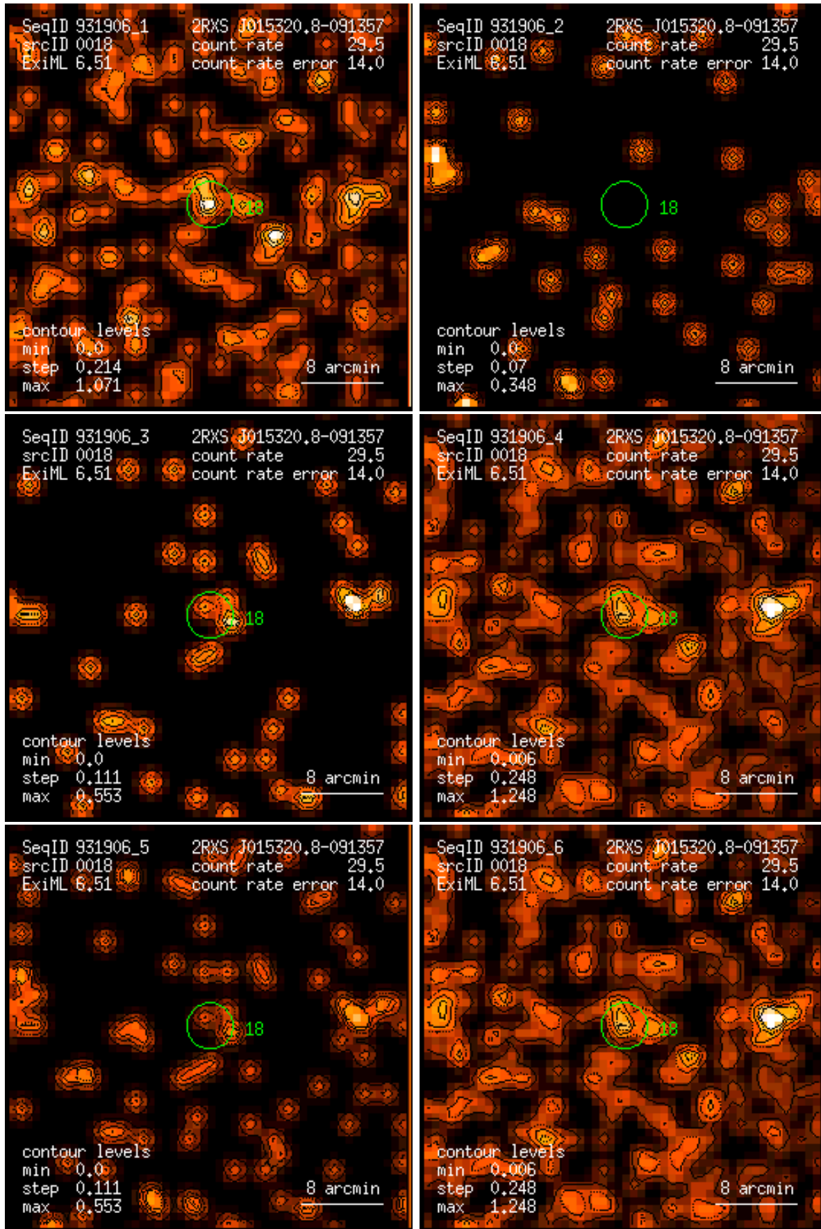
Figure 18: RASS 931906: detection 0018: band rate images, Gaussian filter: (1) PSPC channels 11 – 41, (2) 52 – 90, (3) 91 – 201, (4) 11 – 235, (5) 52 – 201, (6) 11 – 201. Broad band rates in counts/ks. Band rate contour levels in counts/ks/arcmin 2 .
