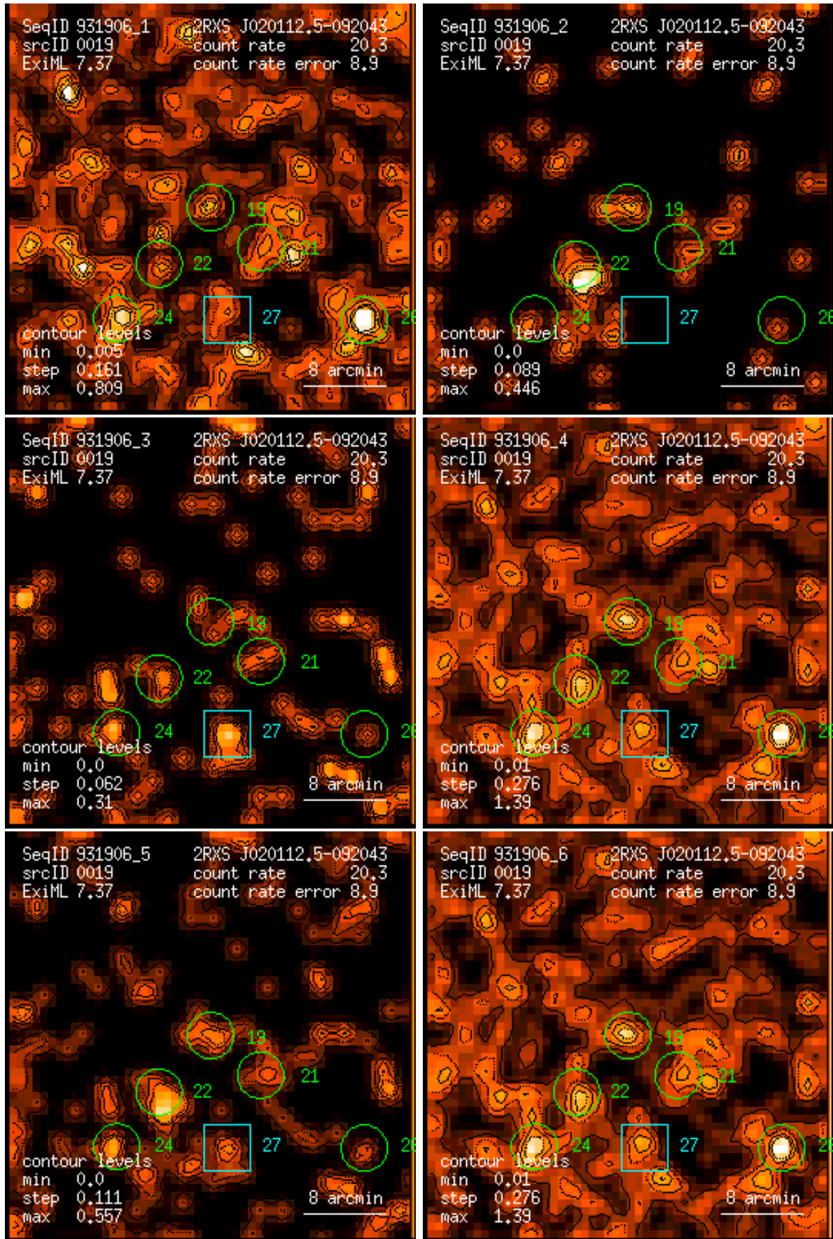
Figure 19: RASS 931906: detection 0019: band rate images, Gaussian filter: (1) PSPC channels 11 – 41, (2) 52 – 90, (3) 91 – 201, (4) 11 – 235, (5) 52 – 201, (6) 11 – 201. Broad band rates in counts/ks. Band rate contour levels in counts/ks/arcmin 2 .
