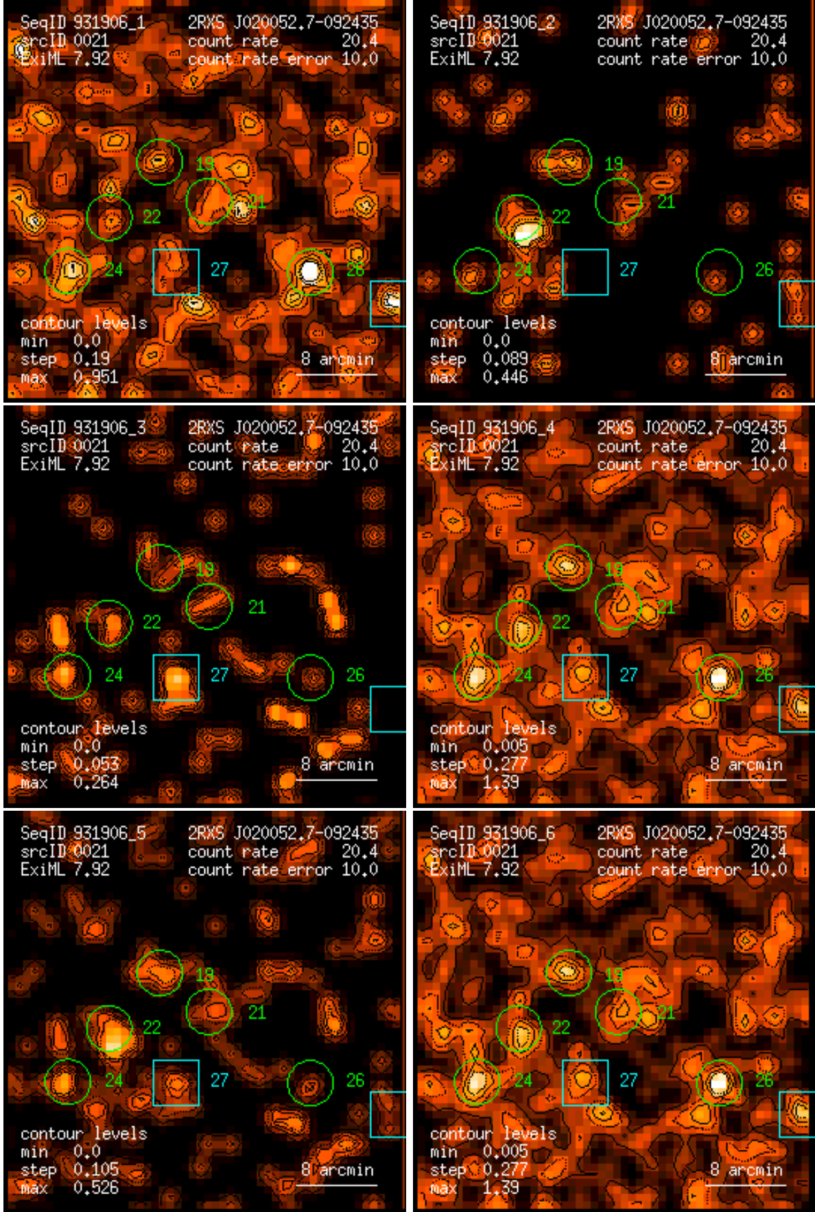
Figure 21: RASS 931906: detection 0021: band rate images, Gaussian filter: (1) PSPC channels 11 – 41, (2) 52 – 90, (3) 91 – 201, (4) 11 – 235, (5) 52 – 201, (6) 11 – 201. Broad band rates in counts/ks. Band rate contour levels in counts/ks/arcmin 2 .
