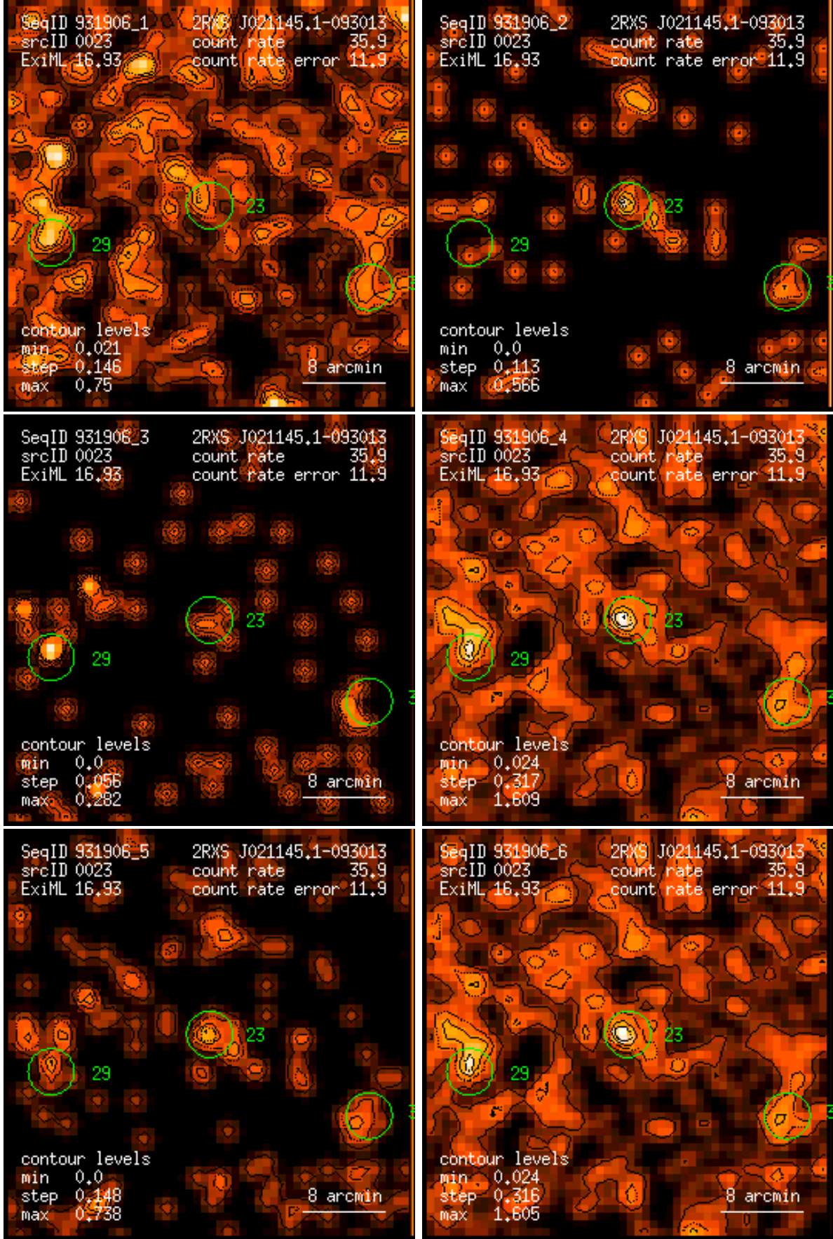
Figure 23: RASS 931906: detection 0023: band rate images, Gaussian filter: (1) PSPC channels 11 – 41, (2) 52 – 90, (3) 91 – 201, (4) 11 – 235, (5) 52 – 201, (6) 11 – 201. Broad band rates in counts/ks. Band rate contour levels in counts/ks/arcmin 2 .
