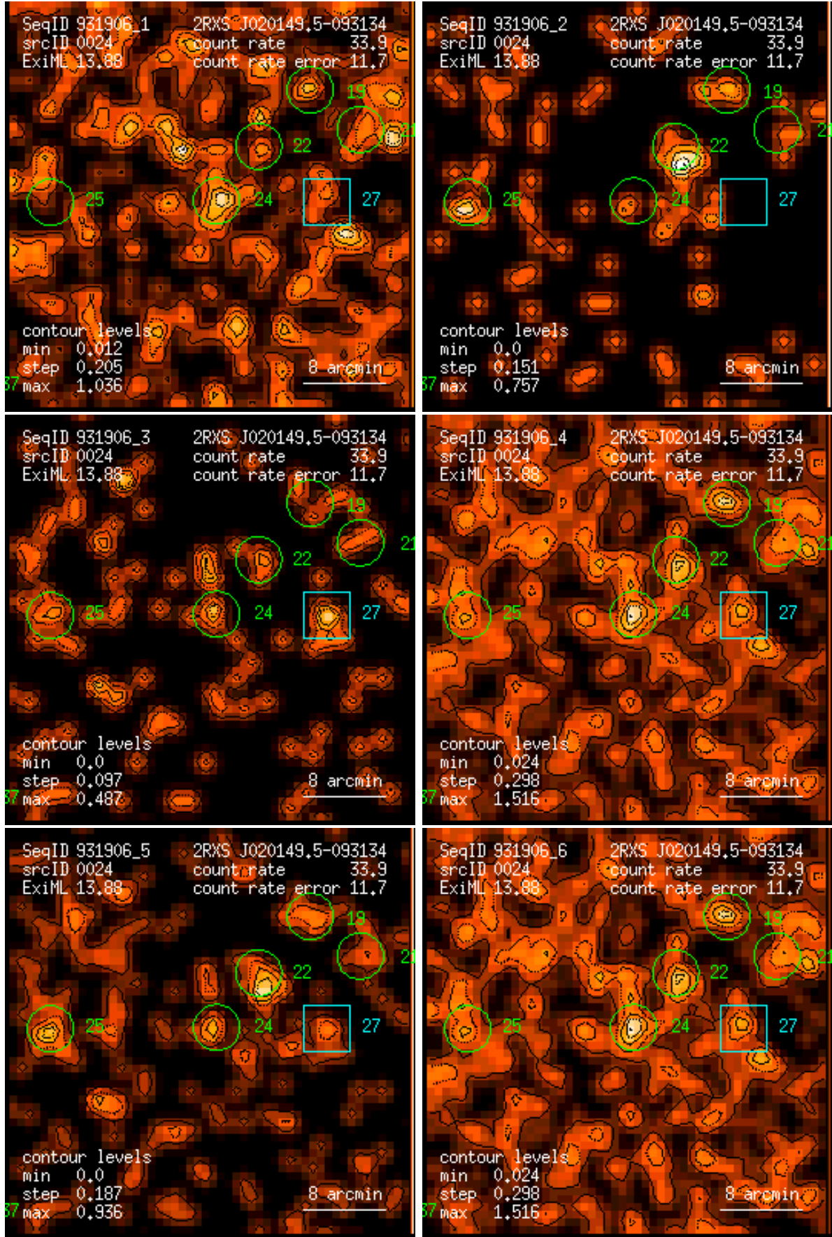
Figure 24: RASS 931906: detection 0024: band rate images, Gaussian filter: (1) PSPC channels 11 – 41, (2) 52 – 90, (3) 91 – 201, (4) 11 – 235, (5) 52 – 201, (6) 11 – 201. Broad band rates in counts/ks. Band rate contour levels in counts/ks/arcmin 2 .
