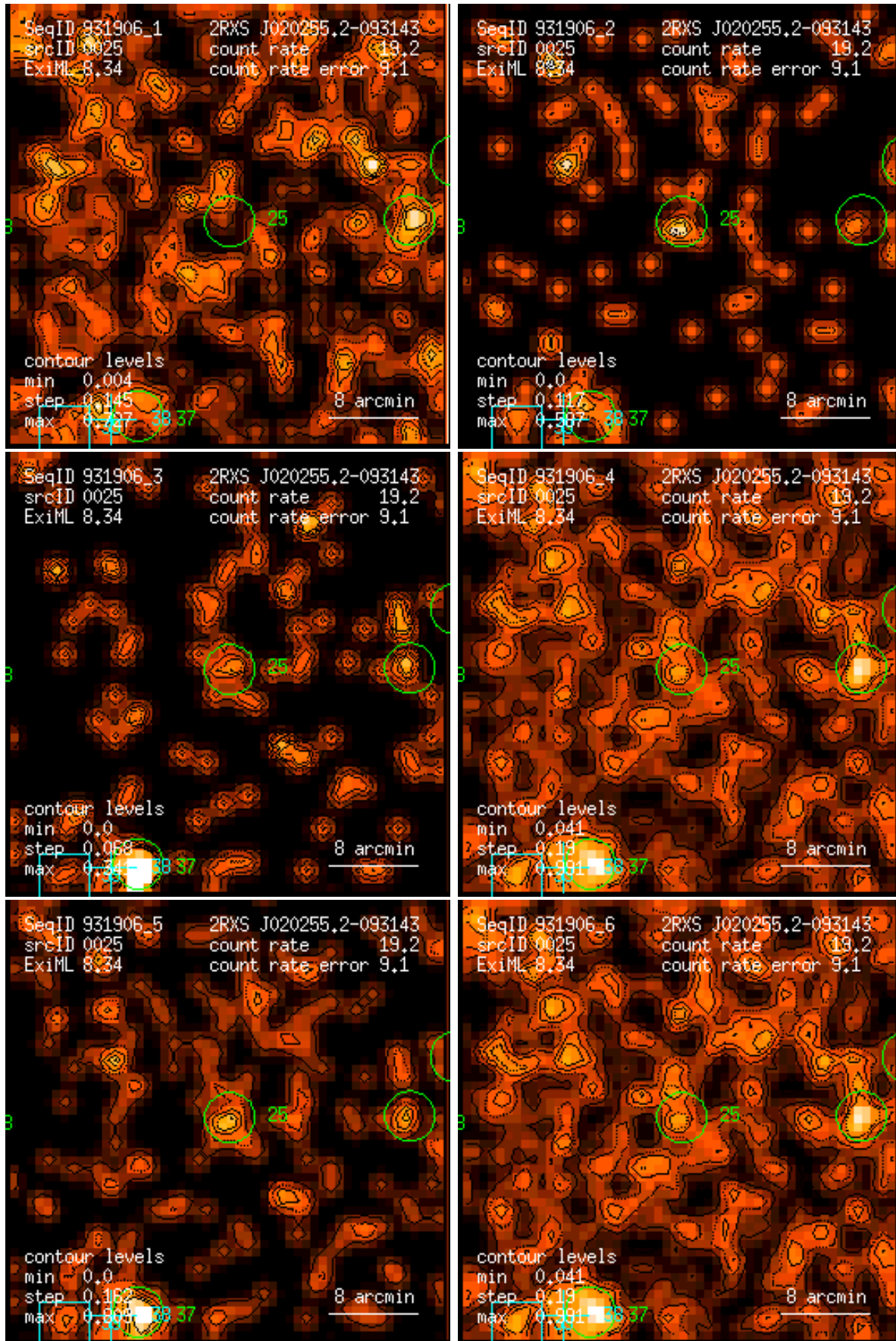
Figure 25: RASS 931906: detection 0025: band rate images, Gaussian filter: (1) PSPC channels 11 – 41, (2) 52 – 90, (3) 91 – 201, (4) 11 – 235, (5) 52 – 201, (6) 11 – 201. Broad band rates in counts/ks. Band rate contour levels in counts/ks/arcmin 2 .
