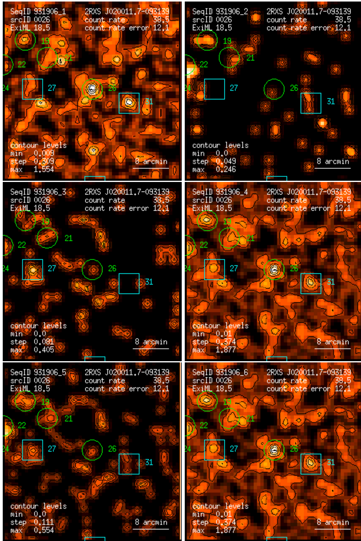
Figure 26: RASS 931906: detection 0026: band rate images, Gaussian filter: (1) PSPC channels 11 – 41, (2) 52 – 90, (3) 91 – 201, (4) 11 – 235, (5) 52 – 201, (6) 11 – 201. Broad band rates in counts/ks. Band rate contour levels in counts/ks/arcmin 2 .
