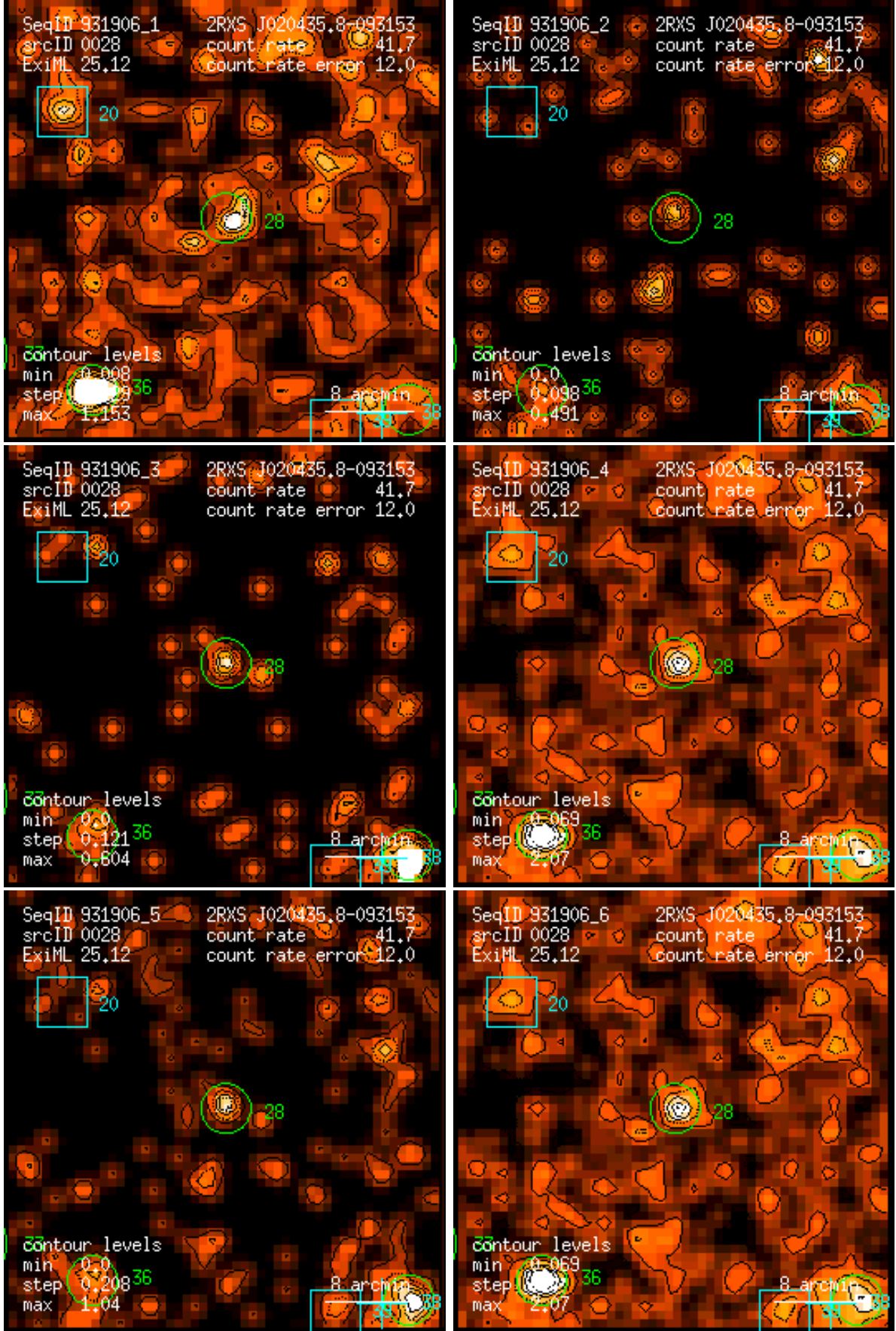
Figure 28: RASS 931906: detection 0028: band rate images, Gaussian filter: (1) PSPC channels 11 – 41, (2) 52 – 90, (3) 91 – 201, (4) 11 – 235, (5) 52 – 201, (6) 11 – 201. Broad band rates in counts/ks. Band rate contour levels in counts/ks/arcmin 2 .
